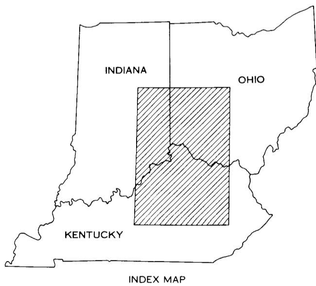
LOCATION MAP AND FENCE DIAGRAM SHOWING COLLECTING LOCALITIES AND STRATIGRAPHIC SECTIONS OF THE BRASSFIELD (SEE TEXT FOR PRECISE LOCATIONS)
