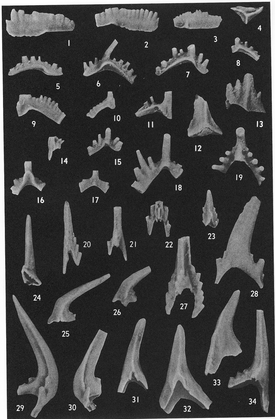
BRASSFIELD CONODONTS
