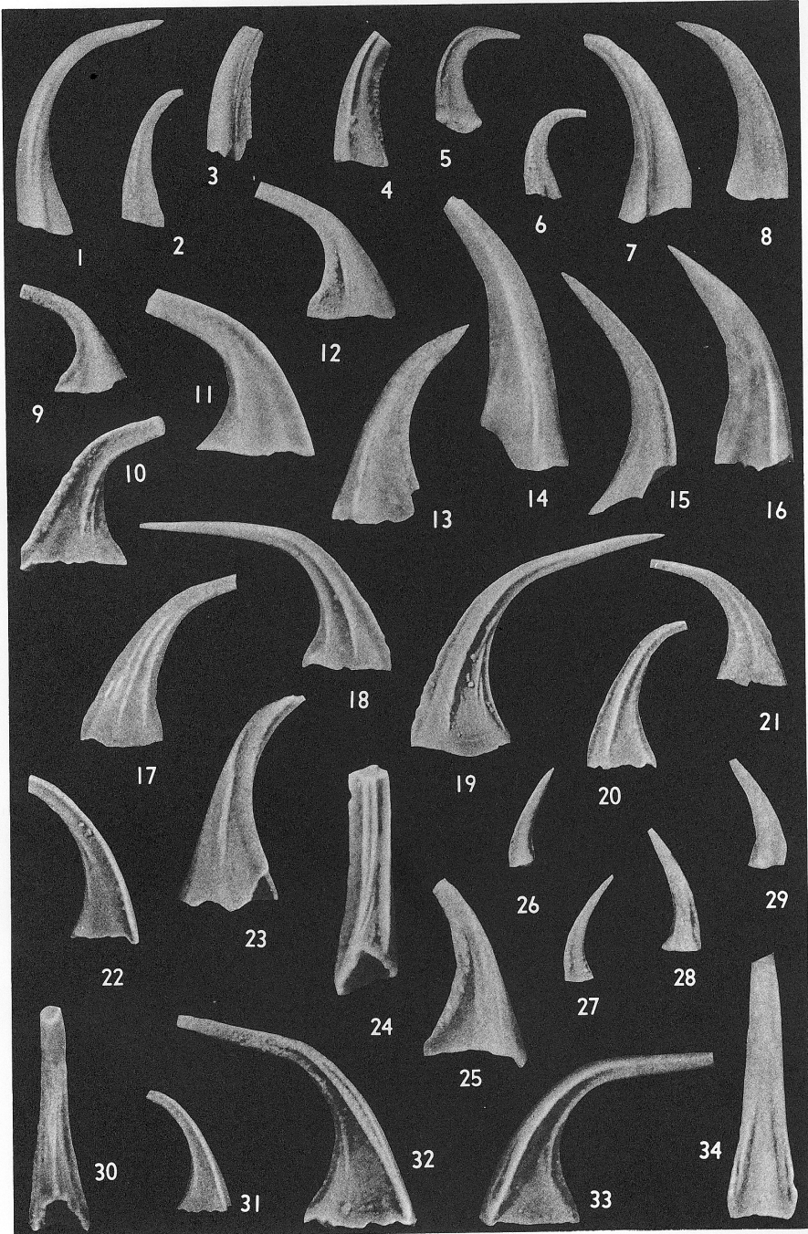
BRASSFIELD CONODONTS
