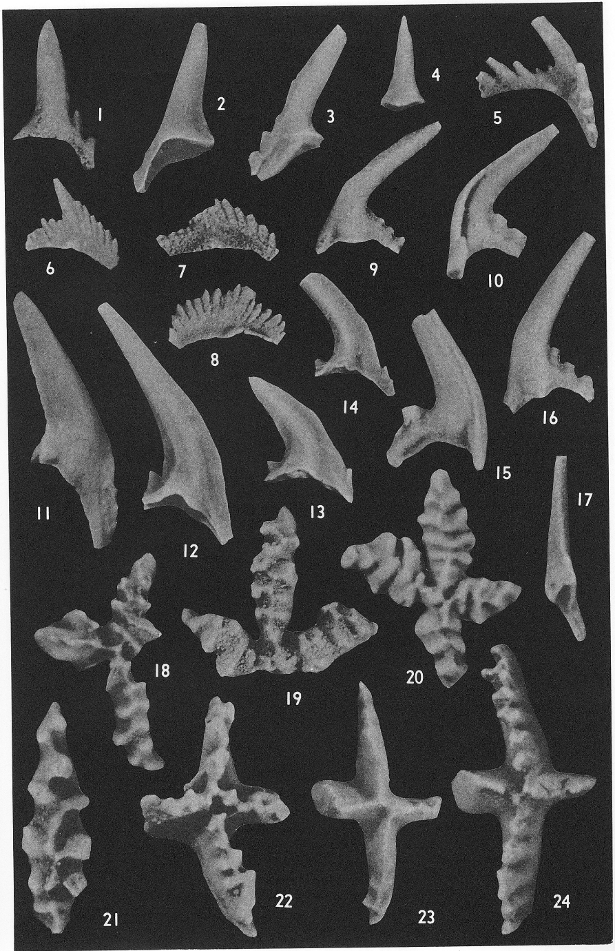
BRASSFIELD CONODONTS
