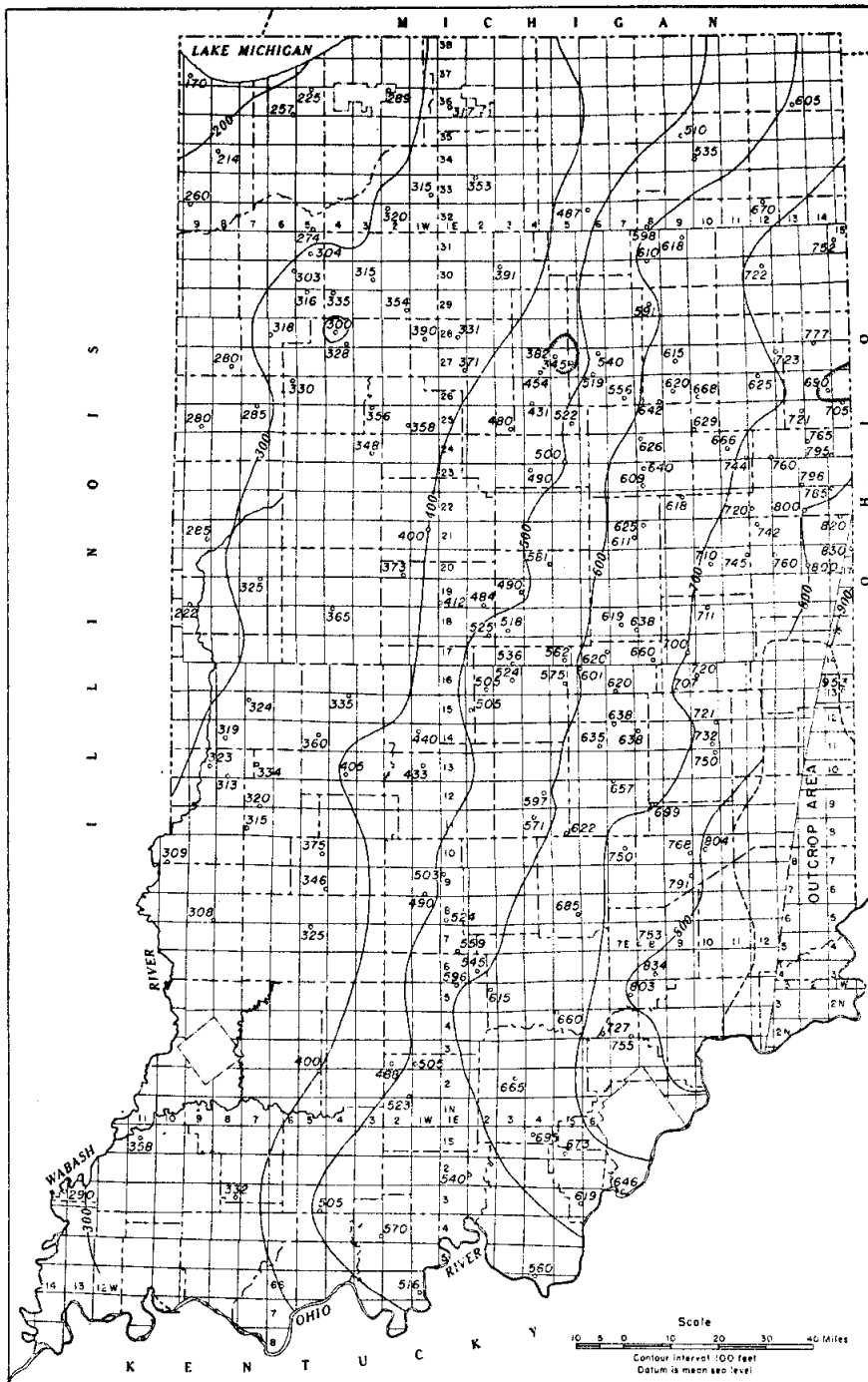
Figure 5. Isopach map of Cincinnati series in Indiana
