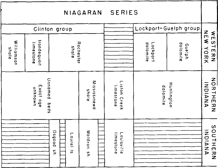
Figure 4. Revised correlation of the Niagaran series of western New York and Indiana
