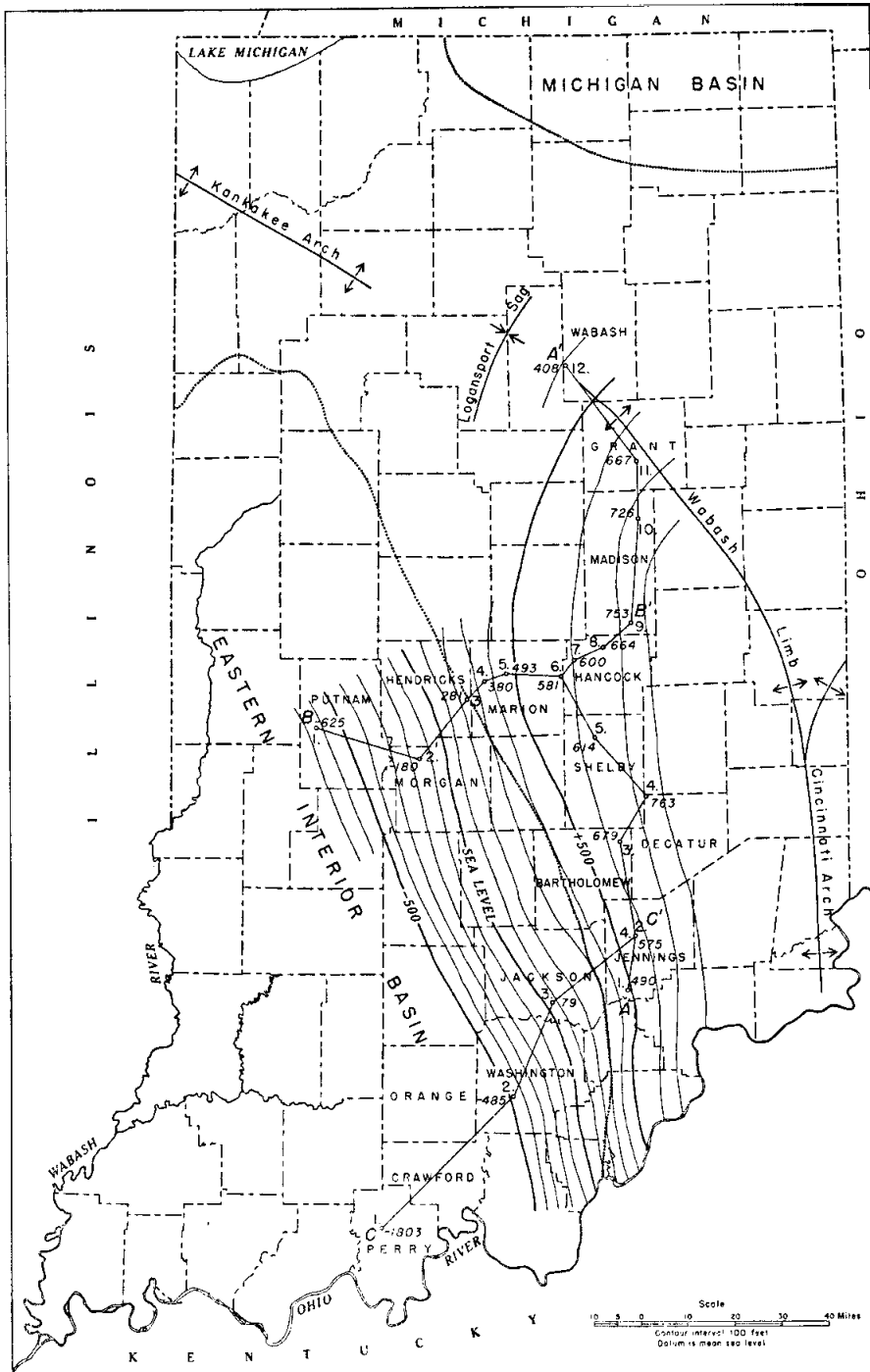
Figure 2. Map of Indiana showing location of wells used in cross sections, regional structural features, and contours on base of Waldron
