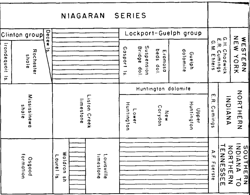
Figure 3. Correlation of Niagaran series of western New York, northern Indiana, and southern Indiana to northern Tennessee AFTER SWARTZ
