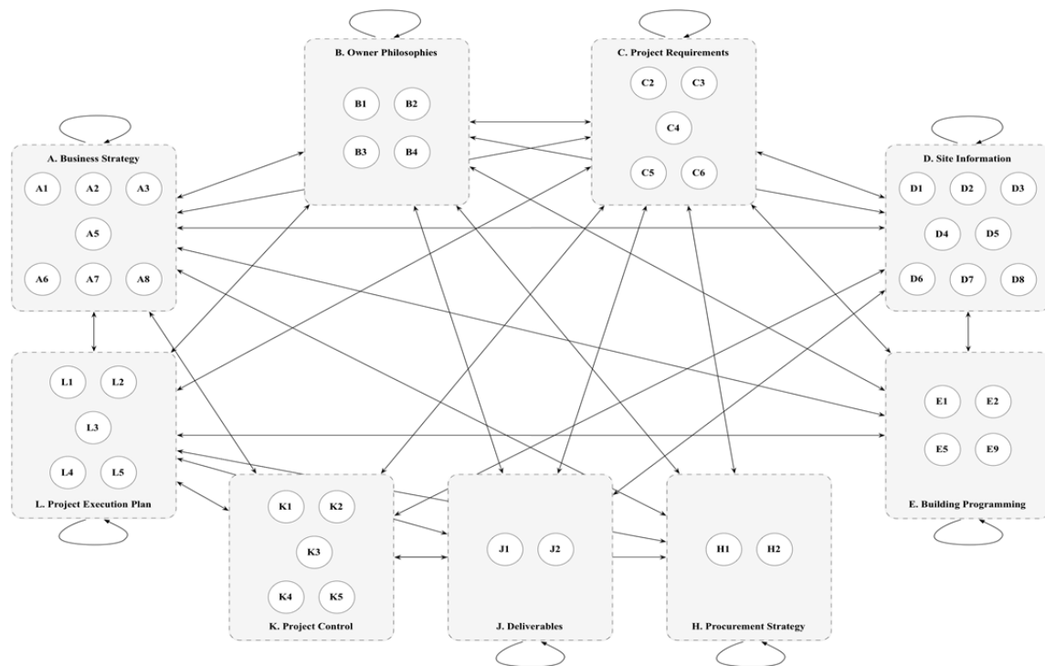
Figure 1: Interrelationships and interactions among elements, ANP model
