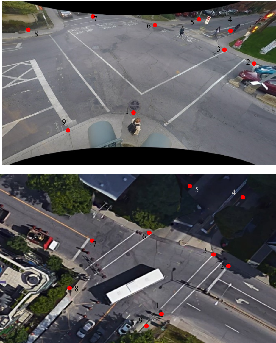
Figure 3-9 Points selected to convert image to world space
