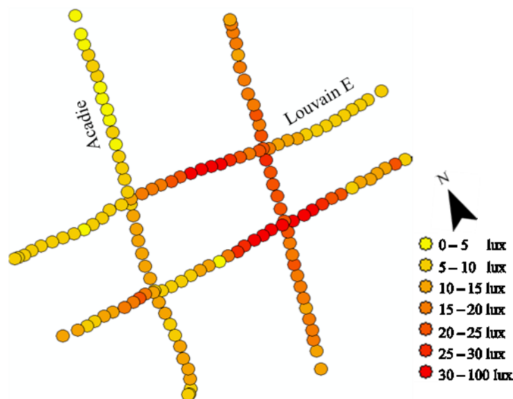
Figure B. 3 Map of the collected illuminance measurements of a sample intersection
