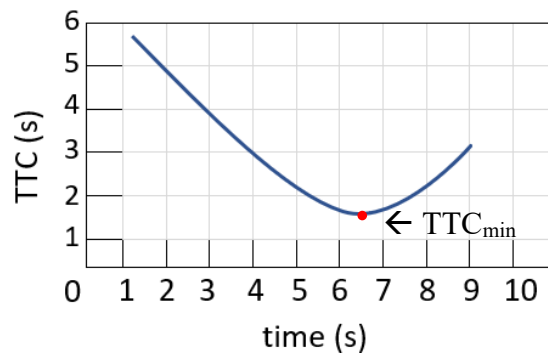
Figure 2-1 TTC curve
