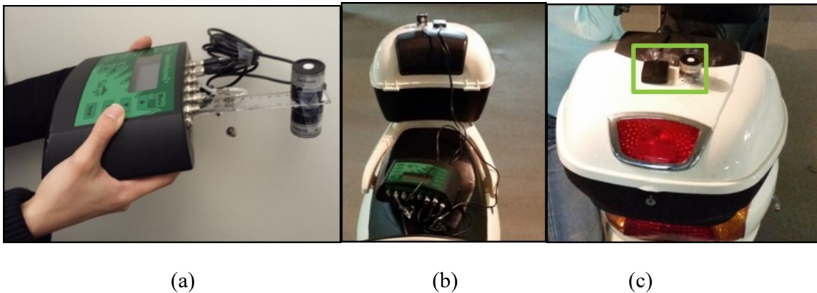
Figure 5-1 a. Data logger and sensor held by the data collector; b. and c. illuminance sensor and GPS mounted on electric scooter
