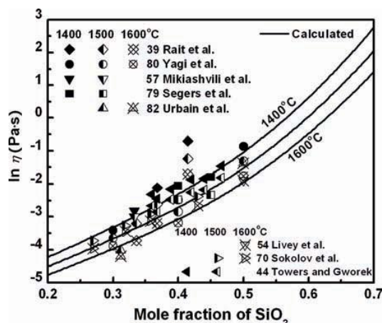
Figure 1. Viscosity of MnO-SiO 2 melts: experimental points [16-23] and calculated lines.
