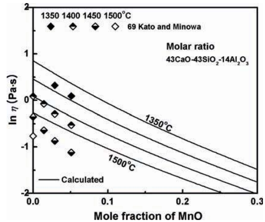
Figure 24. Viscosity of MnO-CaO-Al 2 O 3 -SiO 2 melts at a molar ratio of 43CaO-43SiO 2 -14Al 2 O 3 : experimental points [34] and calculated lines.
