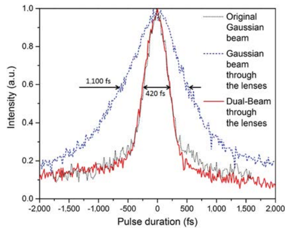
Figure 2. The ultrashort laser pulse duration remains unaffected after been focused using the Dual-Beam technique compared to conventional focusing.
