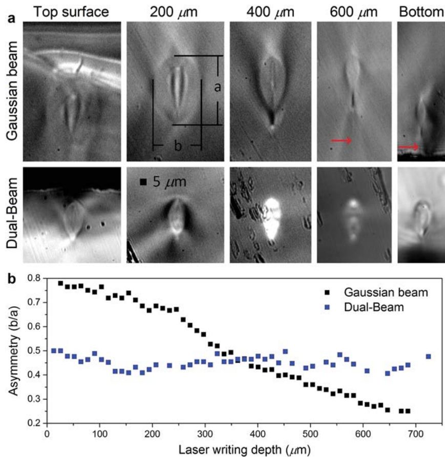
Figure 6. The laser writing depth dependency is strongly reduced using the Dual-Beam technique compared to the conventional focusing technique. (a) Facet view of the waveguides at different depths. Note that the red arrows show weak filaments produced under low energy pulses ( 1 \mu\text{J} ) as discussed earlier. (b) Graph of the measured asymmetry showing the depth of writing dependency.
