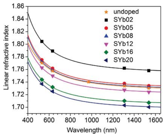
Figure 3. Measured linear refractive index ( n ) of the undoped and \text{Yb}^{3+} -doped glasses as a function of wavelength. The data were fitted by using the Sellmeier's dispersion formula.
