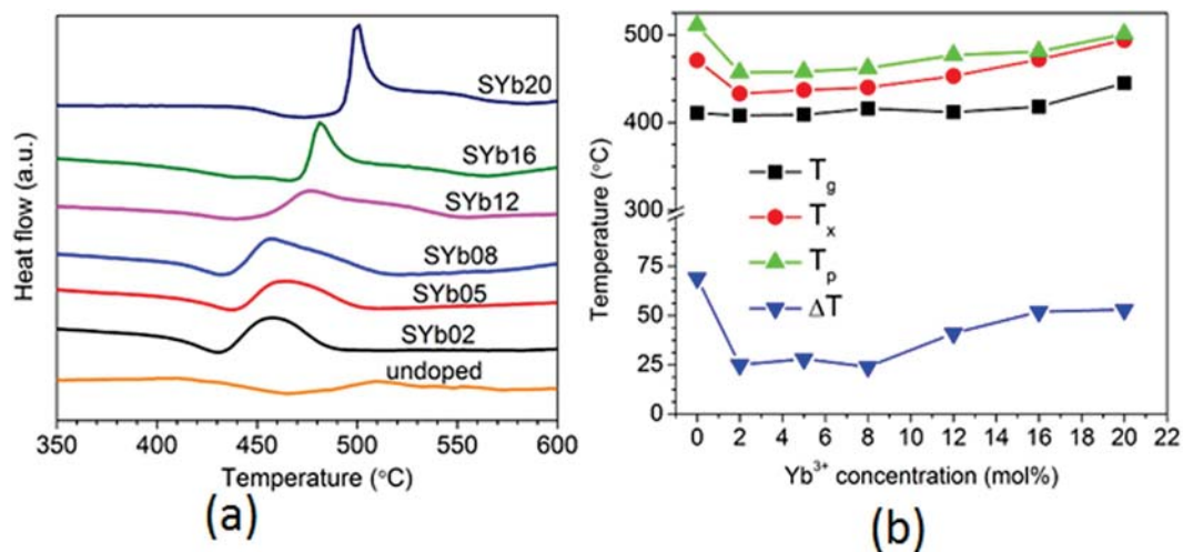
Figure 2. (a) DSC traces of the undoped and \text{Yb}^{3+} -doped 30\text{SiO}_2\text{-}15\text{Al}_2\text{O}_3\text{-(}29\text{-}x\text{)CdF}_2\text{-}22\text{PbF}_2\text{-}4\text{YF}_3\text{-}x\text{YbF}_3 oxyfluoride glasses as a function of \text{Yb}^{3+} concentration ( x ). The thermograms were vertically shifted for better comparison. (b) Variation of T_g , T_x , T_p and \Delta T of the samples under study as a function of \text{Yb}^{3+} concentration.
