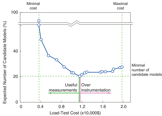
Figure 13. Multi-objective optimization results for the Langensand Bridge.
