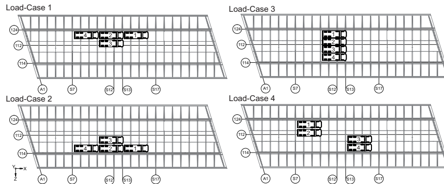
Figure 12. Load-case layout
