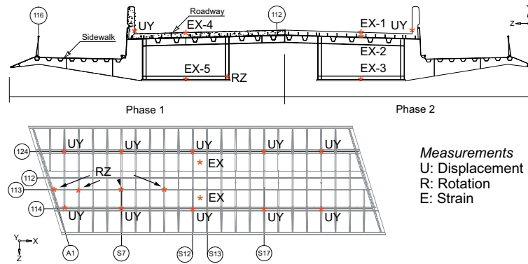
Figure 11. Langensand Bridge cross-section and sensor layout
