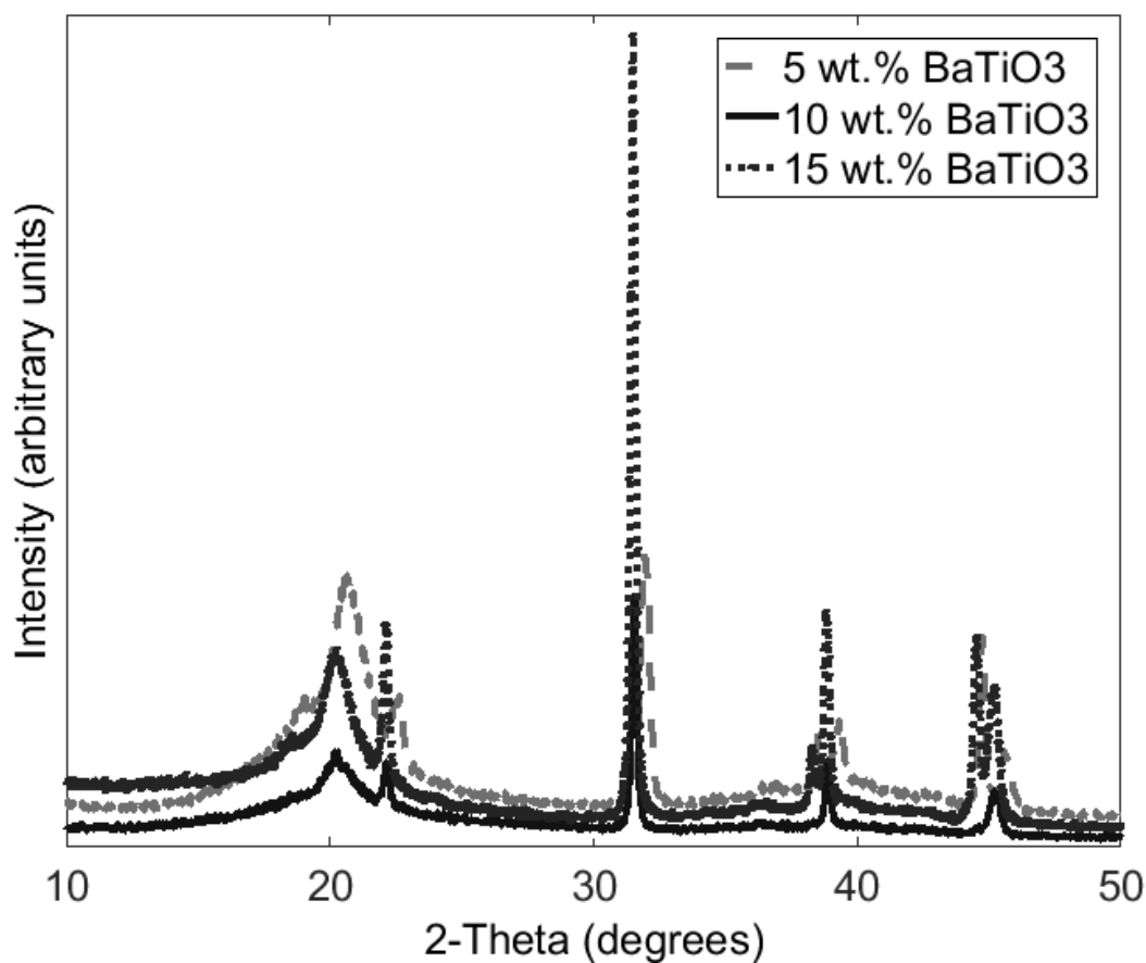
Figure 4.14: X-ray diffractogram of nanocomposite films prepared by ball-mill mixing with 5, 10 and 15 wt.% BaTiO 3 nanoparticles in PVDF
