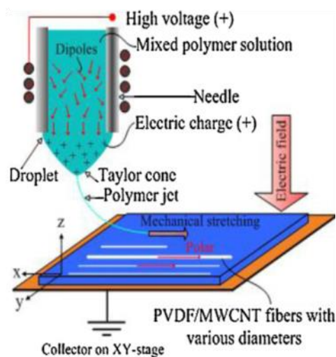
Figure 2.4: Schematic of NFES [35]
