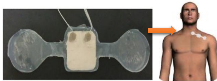
Figure 2.20: Photograph of sensor patch (transparent = PDMS and opaque = PVDF) [117]
