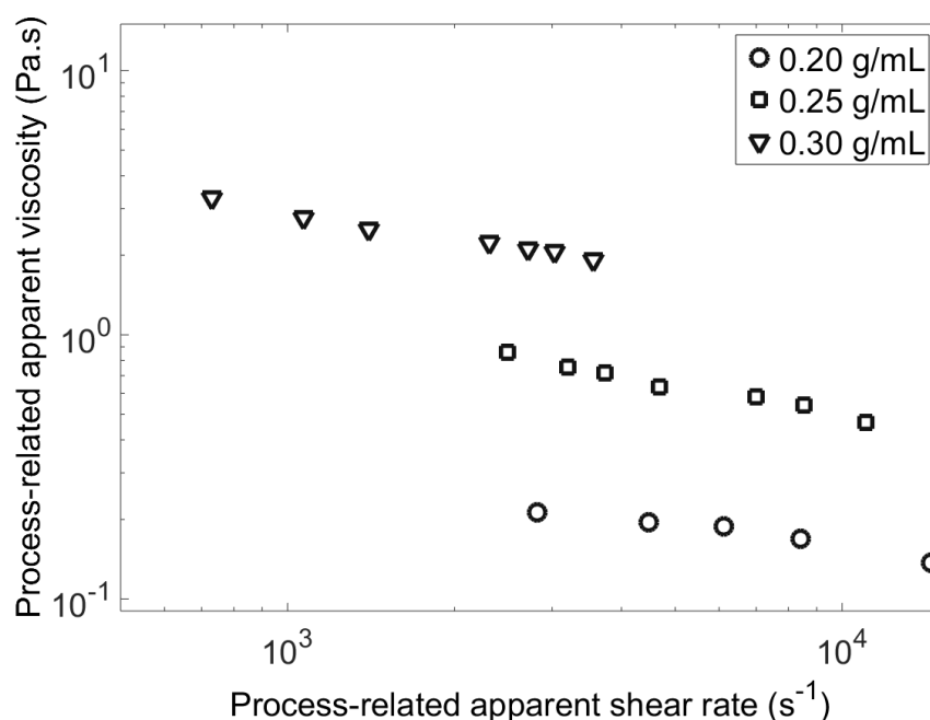
Figure 4.8: Viscosity as a function of shear rate during the printing process for 0.20, 0.25, and 0.30 \text{g mL}^{-1} of the ball-milled nanocomposite with 10 wt.% BaTiO 3 NPs (printing parameters: 0.5 \text{ mm s}^{-1} with a 100 \mu\text{m} nozzle)
