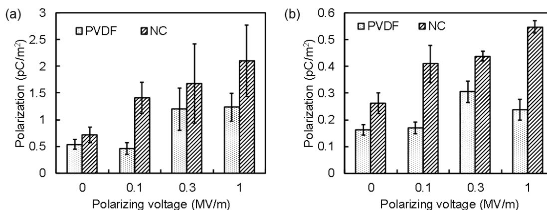
Figure 5.6: Piezoelectric outputs of P and NC sensors fabricated with electric fields 0, 0.1, 0.3 and 1 \text{MV m}^{-1} . (a) Average of 5 different samples, and (b) average of a single sample tested 5 times
