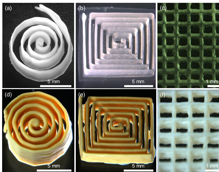
Figure 5.9: Optical images of 3D structures fabricated with P (a) a 40 layer circular spiral (0.25 g mL -1 PVDF solution; 0.5 MPa; 1 mm s -1 ; 100 μm); (b) a 40 layer square spiral (0.25 g mL -1 PVDF solution; 0.5 MPa; 1 mm s -1 ; 100 μm); (c) a 9 layer scaffold (0.3 g mL -1 PVDF solution; 0.2 MPa; 3 mm s -1 ; 150 μm). Structures fabricated with NC: (d) a 40 layer circular spiral (0.25 g mL -1 NC solution; 0.5 MPa; 1 mm s -1 ; 100 μm); (e) a 40 layer square spiral (0.25 g mL -1 NC solution; 0.5 MPa; 1 mm s -1 ; 100 μm); (f) a 9 layer scaffold (0.3 g mL -1 NC solution; 1.3 MPa; 13 mm s -1 ; 250 μm)
