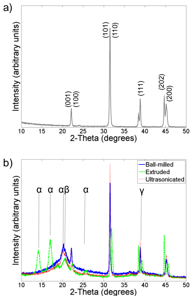
Figure 4.4: X-ray diffractogram of (a) \text{BaTiO}_3 NPs and (b) nanocomposites of 10 wt.% \text{BaTiO}_3 NPs and PVDF prepared by ball-milling, extrusion and sonication (printing parameters: \sim 1 MPa at 20 \text{ mm s}^{-1} with a 100 \mu\text{m} nozzle)
