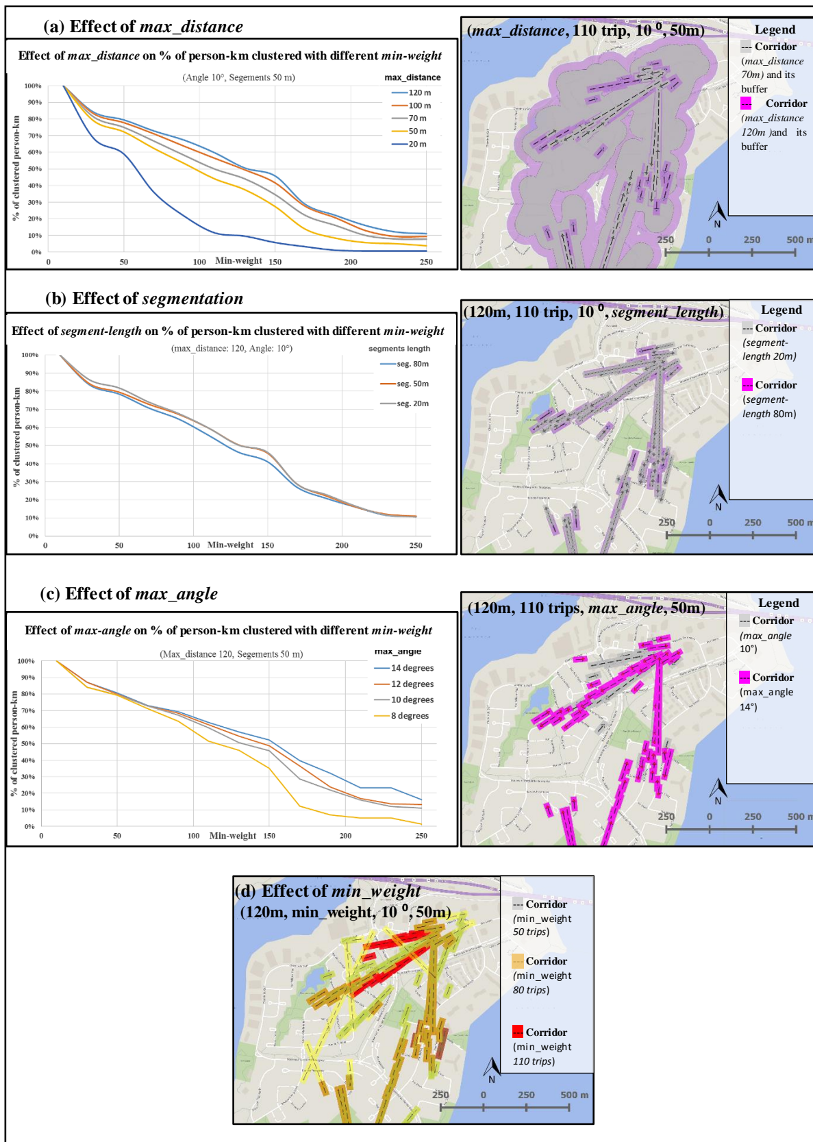
Figure 5.9: Sensitivity analysis of TraClus-DL vs input values
