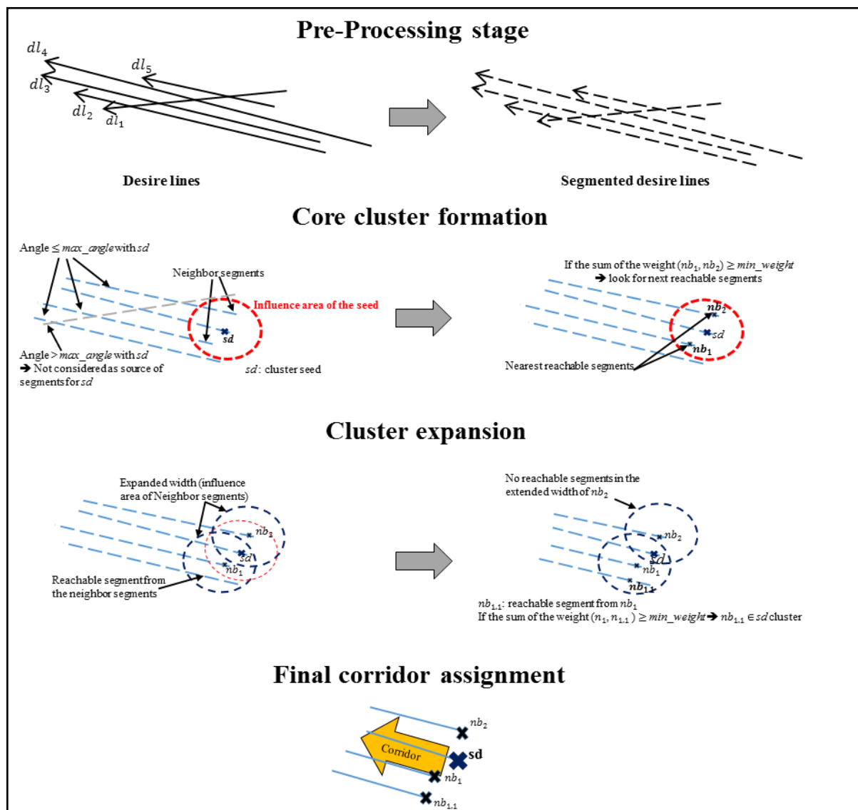
Figure B.3: TraClus-DL processing stages
