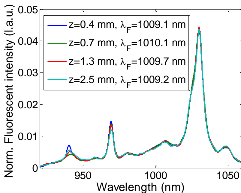
Figure 3-7: Photoluminescence spectra of a 3% Yb:YAG crystal, after correction for reabsorption. The labels indicate at which depth, z the uncorrected data is collected.
