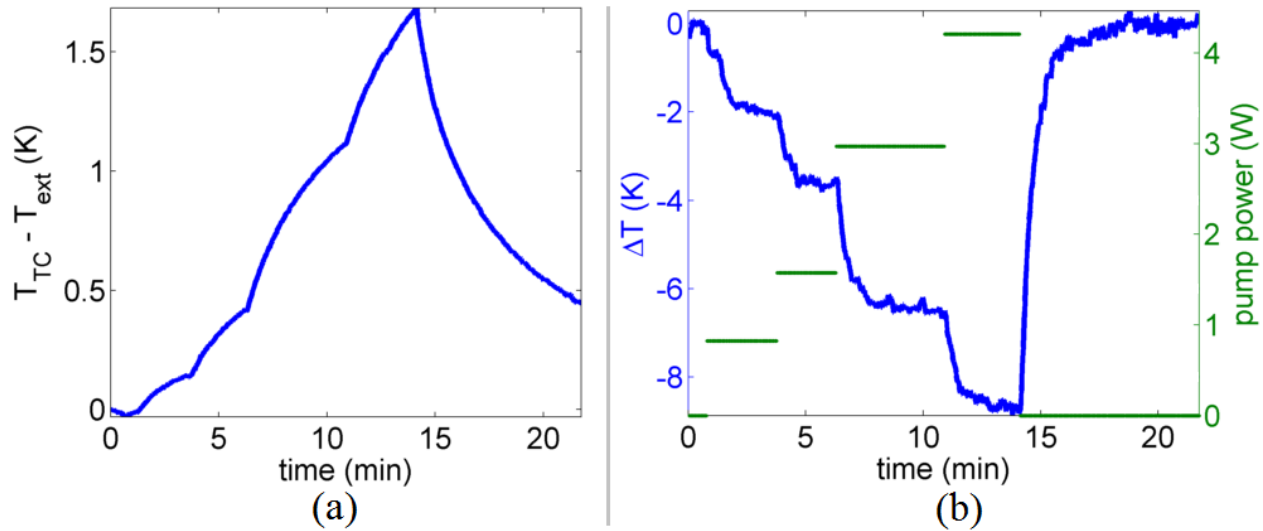
Figure 5-10 Temperature dynamics as the laser pump power is increased from 0 W up to 4.2 W. (a) The chamber temperature variation, measured by the thermocouple. (b) The difference between the temperature of the Yb:YAG crystal measured by the FBG and the chamber temperature. Before 0 s the crystal was shortly pumped for test purposes, which explains the finite temperature difference at 0 s, but which stabilized after \sim 1 min.
