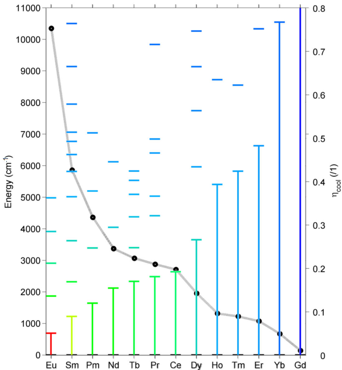
Figure 2-2: Left axis, colored data: Dieke energy diagram – truncated to 11000 \text{ cm}^{-1} – for trivalent lanthanide ions, ordered by their first excited state electronic energy gap. The first electronic excited level is indicated by a column below it, and the colors correspond qualitatively to the photon necessary to excite that level. Right axis, black circles: ideal cooling efficiency, considering a reference anti-Stokes shift of 521 \text{ cm}^{-1} , i.e. 2.5 \times k_B T at room temperature. Position of the energy levels from [102].
