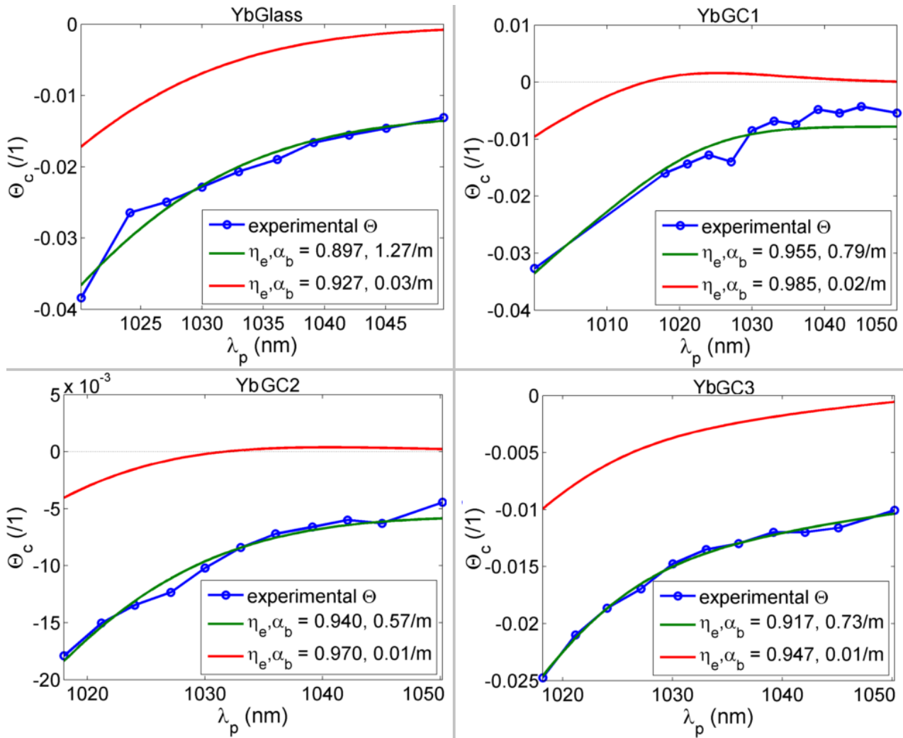
Figure 6-17: Cooling figure-of-merit spectra of the samples. In red: theoretical \Theta_c based on the experimental data with an improvement \Delta\eta_{ext} = 0.03 and \alpha_{b,new} = \alpha_b/50 .
