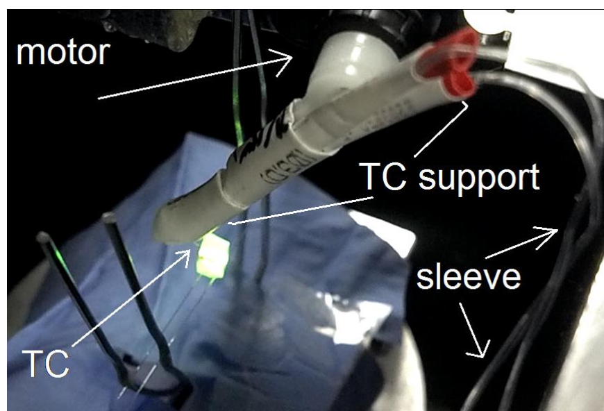
Figure 4-7: Photograph of the inside of the cooling chamber in initial tests. A small servo-motor controls the position of the thermocouple support. The 1-mm 3 sample (green) is pumped on purpose so that it is easier to see the thermocouple due to the green light scattering.
