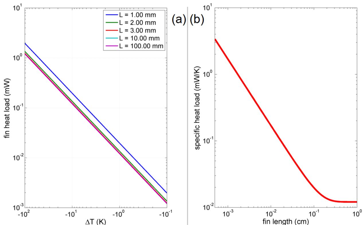
Figure 5-3: Total heat load of the fin to the sample as a function of the temperature difference between the sample and the environment (a), and as a function of the length (b) of the 125 μm-diameter silica fin.
