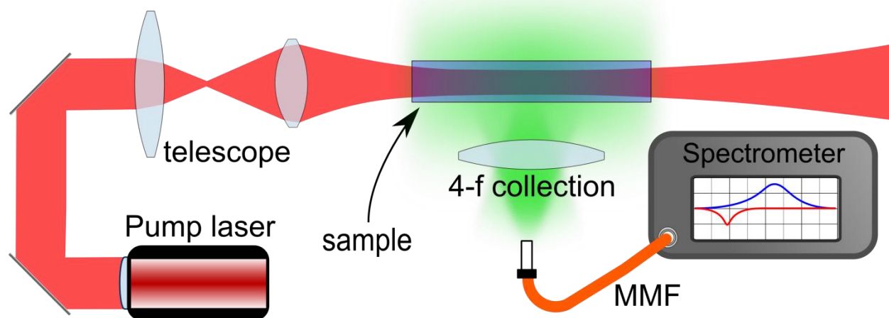
Figure 3-1: Diagram of the general optical setup for measurement of the photoluminescence spectra. The sample is placed at the waist of a collimated beam and a collection lens is placed at a 90^\circ angle at a distance 2f , where f is the focal length of the lens. The fluorescence is thus focused into a multimode fiber at a distance 2f from the lens, and directed to an optical spectrometer.
