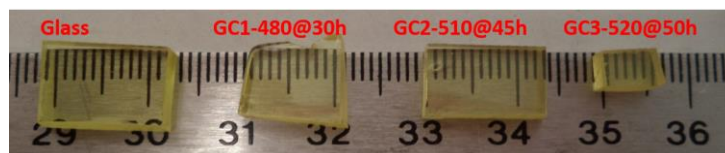
Figure 6-7: Photograph of the 2 mol. % Yb-doped glass and the glass-ceramic samples fabricated from a duplicate of the glass, after different annealing times.
