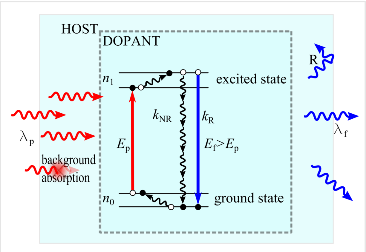
Figure 2-1: Simplified diagram of the optical cooling process upon absorption of a photon and emission of a blue-shifted photon. Also shown are the most important processes which can occur within the material. Incoming photons of wavelength \lambda_p (red arrows) enter the host material, and some of them can suffer multiple scattering and be absorbed in unwanted impurities (background absorption). The remaining photons interact with the dopant ion, exciting electrons from the ground manifold n_0 to the excited manifold n_1 , where they are thermalized within the manifold. The electrons in n_1 return to the ground state by a nonradiative path through multiphonon (black arrows) relaxations at a rate k_{NR} , or by a radiative path, i.e. emitting photons at a rate k_R (blue line). The emitted photons (blue arrows) of wavelength \lambda_f can escape the material, or can be trapped as well and reabsorbed in the sample volume or reflected (R) at the surface. The electrons undergo thermalization, absorbing phonons from the lattice, and end up at a sublevel (horizontal lines) following a Boltzmann distribution. The emitted photons, as well as the reflected ones, can undergo all the same processes as the incoming photons.
