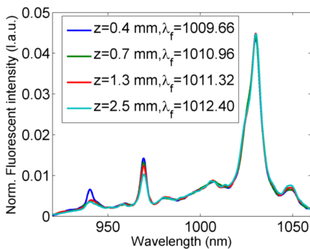
Figure 3-6: Depth-dependent photoluminescence spectra of a 3% Yb:YAG crystal.
