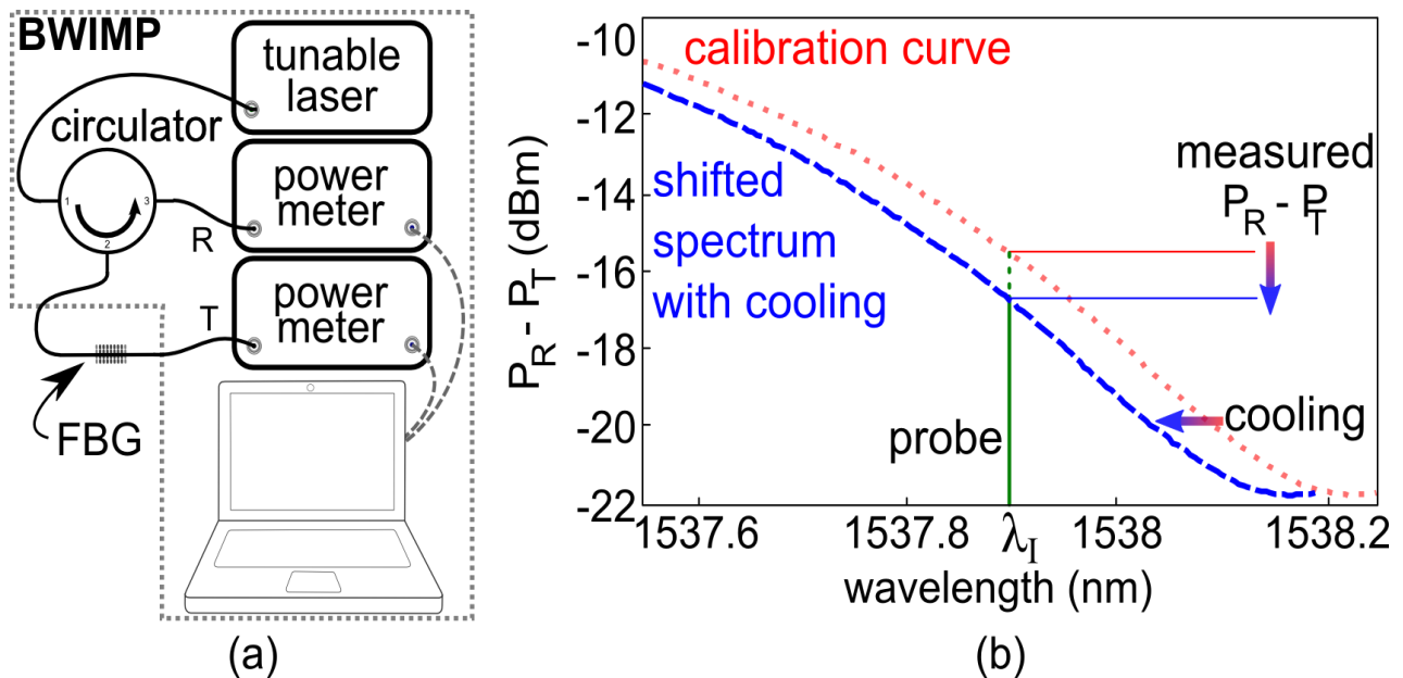
Figure 4-10: FBG interrogation method based on reflected and transmitted power. (a) Experimental setup. (b) Measured reflection/transmission power spectra from the FBG before the cooling experiment (right). The curve on the left is a representation of the shifted spectra after a temperature drop, and the corresponding power change measured by the power meters when the fiber is interrogated at a single wavelength \lambda_T (continuous line). Notice that at the bottom of the P_R - P_T , one cannot assign a single wavelength to a given measured power.
