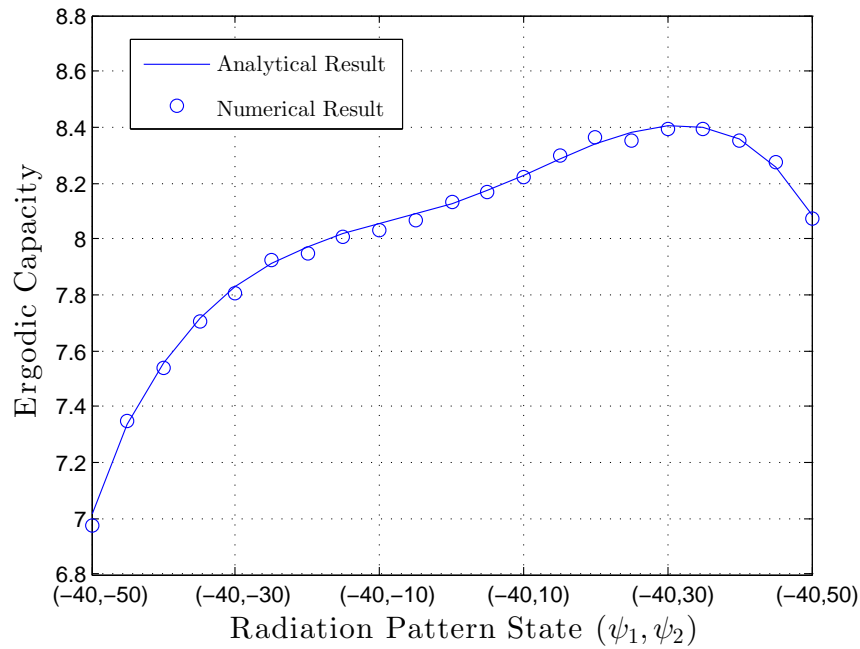
Figure 5.10 Ergodic channel capacity of a 2 \times 2 RE-MIMO system at high SNR for a bi-modal truncated Laplacian PAS with \phi_0^1 = -40^\circ , \phi_0^2 = 40^\circ , P_1 = -1.7 dB, and P_2 = -5 dB.
