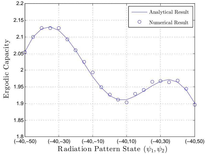
Figure 5.9 Ergodic channel capacity of a 2 \times 2 RE-MIMO system at low SNR for a bi-modal truncated Laplacian PAS with \phi_0^1 = -40^\circ , \phi_0^2 = 40^\circ , P_1 = -1.7 dB, and P_2 = -5 dB.
