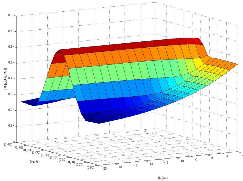
Figure 5.5 Covariance coefficient with AS = 10^\circ and \psi_1 = \phi_0^1 = 0^\circ as a function of \psi_2 and \beta_2 .
