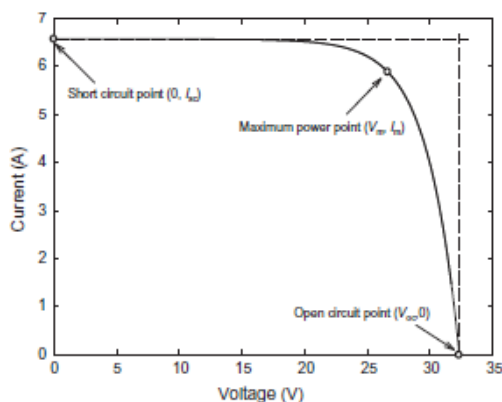
Fig. 2. I - V characteristic curve of an ideal PV cell.
