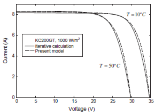
Fig. 4. I - V curve of the KC200GT at E = 1000 W/m 2 .
