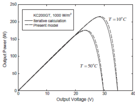
Fig. 6. P - V curve of the KC200GT at E = 1000 W/m 2 .
