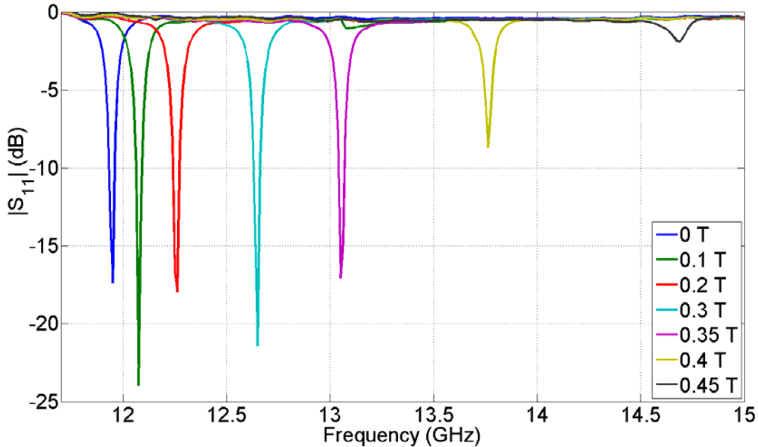
Figure 3.2-7: Measurement results displaying the resonant peaks of a double ferrite slabs loaded cavity resonator versus frequency.
