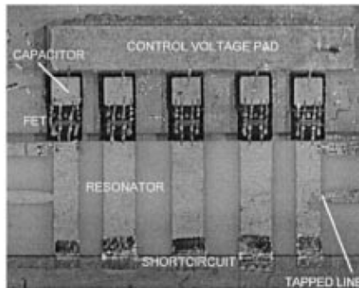
Figure 1.1-3: Fabricated filter prototype [Torregrosa-Penalva, et al., (2002)].
