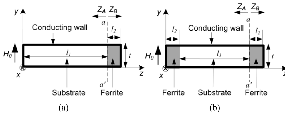
Figure 3.2-4: Cross-sectional view of the SIW cavity loaded with (a) a single ferrite slab and (b) two ferrite slabs along the side walls.
