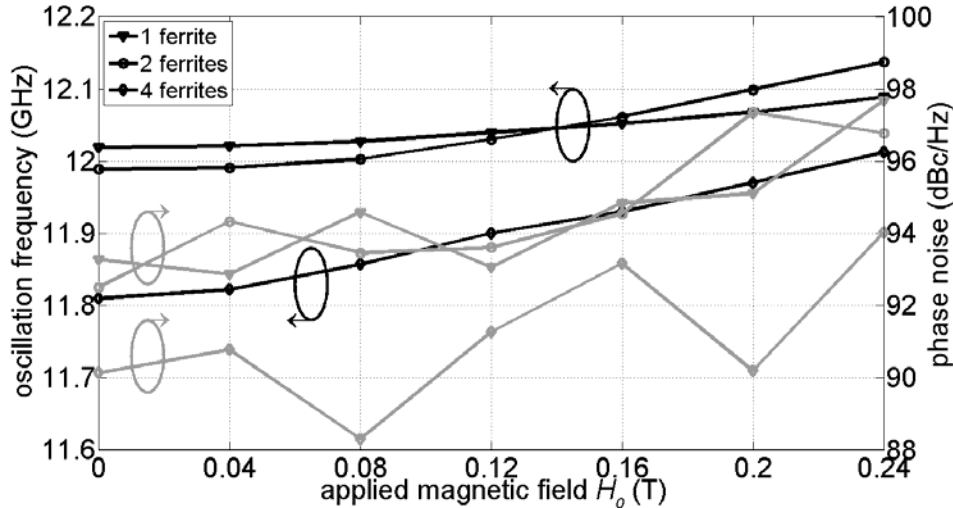
Figure 3.3-25: Oscillator frequency tuning range and phase noise performance versus applied magnetic bias.
