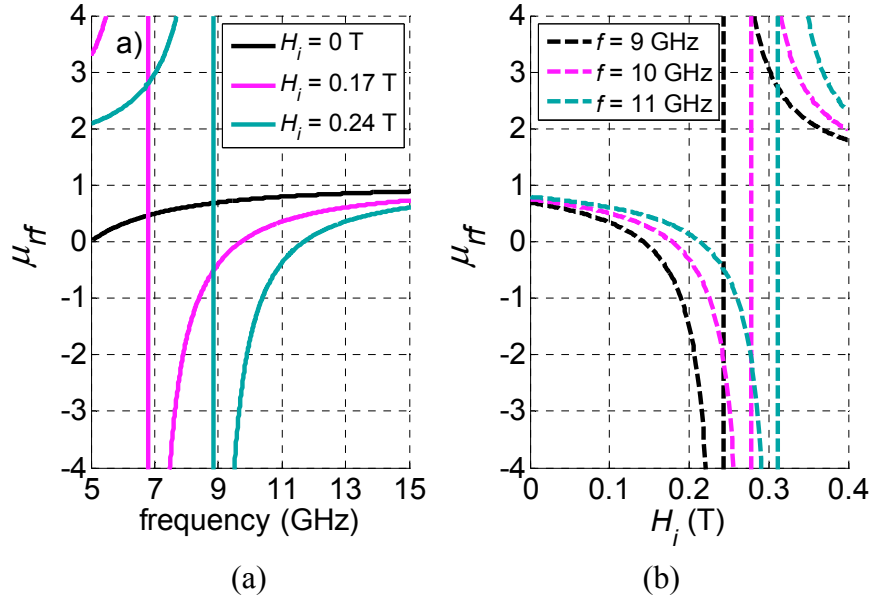
Figure 3.4-30: Calculated \mu_{rf} of YIG ferrite, a) versus frequency at internal magnetic fields H_i = 0 T, 0.17 T and 0.24 T, b) versus internal magnetic field H_i at frequencies f = 9 GHz, 10 GHz and 11 GHz.
