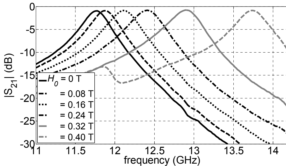
Figure 3.3-19: Measurement results of multi-layer cavity resonator.
