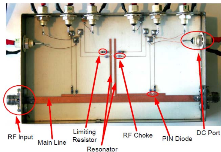
Figure 1.1-1: Photograph of the fabricated switchable band-pass filter [Brito-Brito, et al. (2008)].
