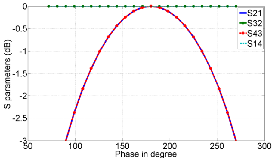
Figure 5.4-14: Calculated S-parameters of an ideal four-port circulator.
