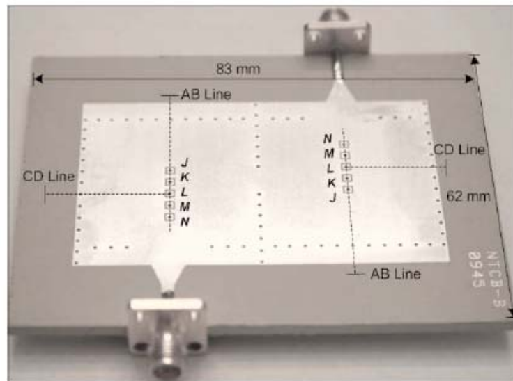
Figure 1.1-2: Fabricated SIW filter with via posts islands for the connection of PIN diodes [Armendariáz, Sekar, and Entesari (2010)].
