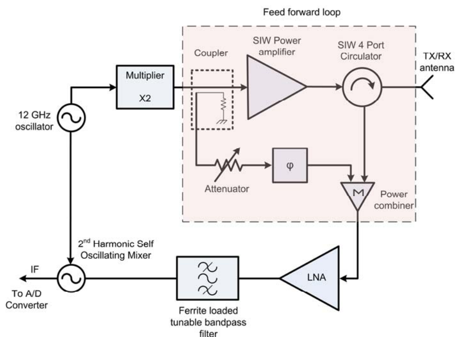
Figure 0.1-3: A schematic of radar system design
