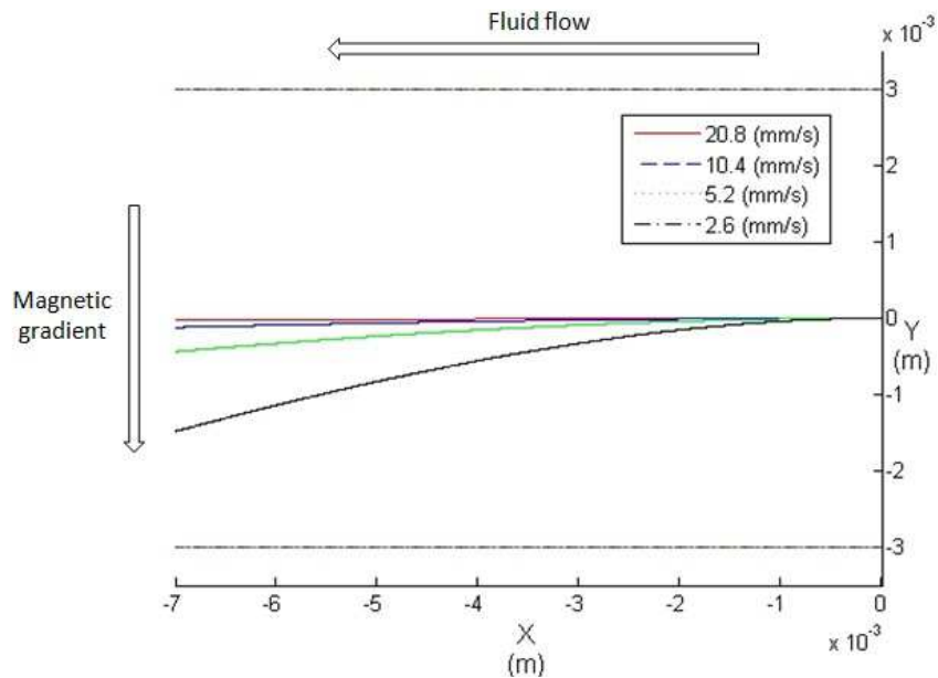
Figure 3-7 Simulated individual microparticle's deflection patterns. Flow velocities considered are 20.8, 10.4, 5.2 and 2.6 mm/s (from top to bottom in the graphic).
