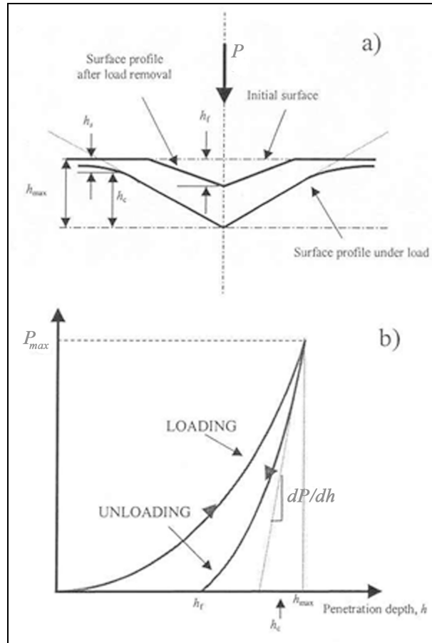
Figure 3.13: Depth-sensing indentation: (a) surface profile under indentation and (b) typical load-displacement curve (adapted from [185]).
