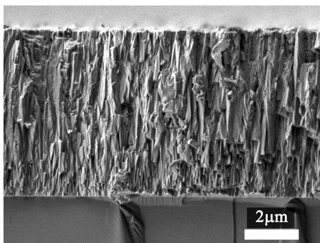
Figure 6.7: Cross-sectional SEM micrograph of the CrN monolithic coating.
