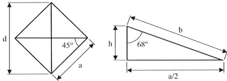
Figure 3.12: Geometrical description of a Vickers type indenter [185].
