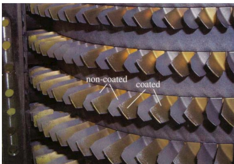
Figure 1.3: GE T64 jet engine compressor with half the blades coated with a TiN-based multilayer coating [7].
