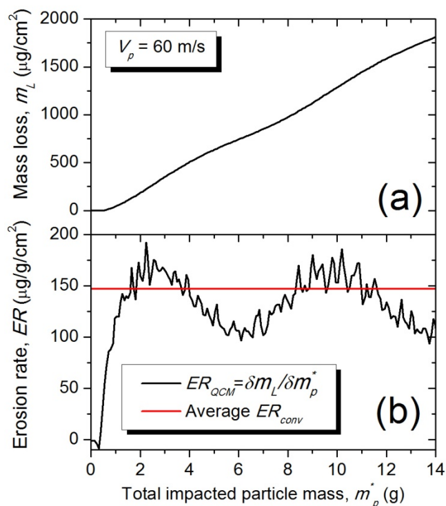
Figure 6.11: SPE of a CrN/Cr multilayer coating: (a) m_L vs. m_p^* , and (b) ER vs. m_p^* .
