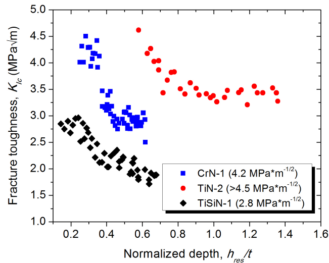
Figure 5.11: K_{IC} for the three coatings deposited on c-Si as a function of h_{res}/t .
