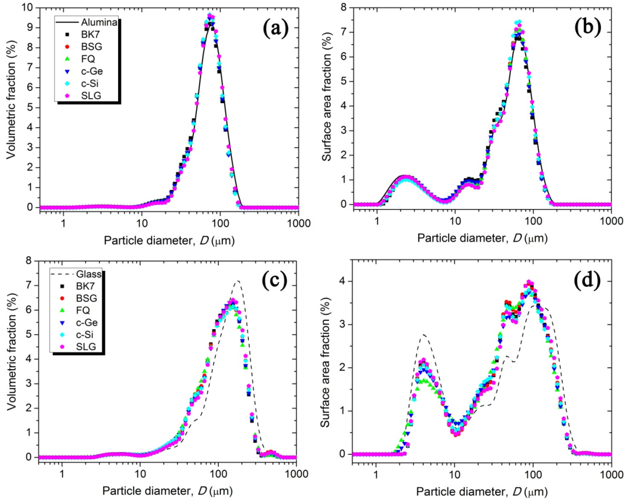
Figure 4.8: Effect of SPE at V_p = 75 m/s on the alumina powder volumetric (a) and surface area (b) distributions, and on the glass powder volumetric (c) and surface area (d) distributions.
