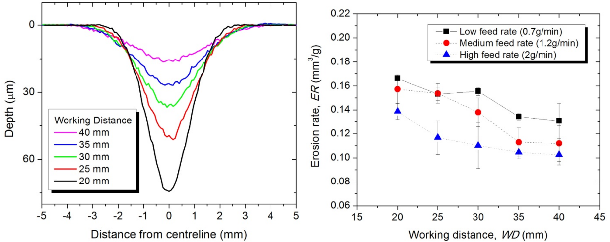
Figure 5.6: Effect of WD on SPE: (a) Erosion scar profiles and (b) Measured ER on c-Si at V_p = 45 m/s.
