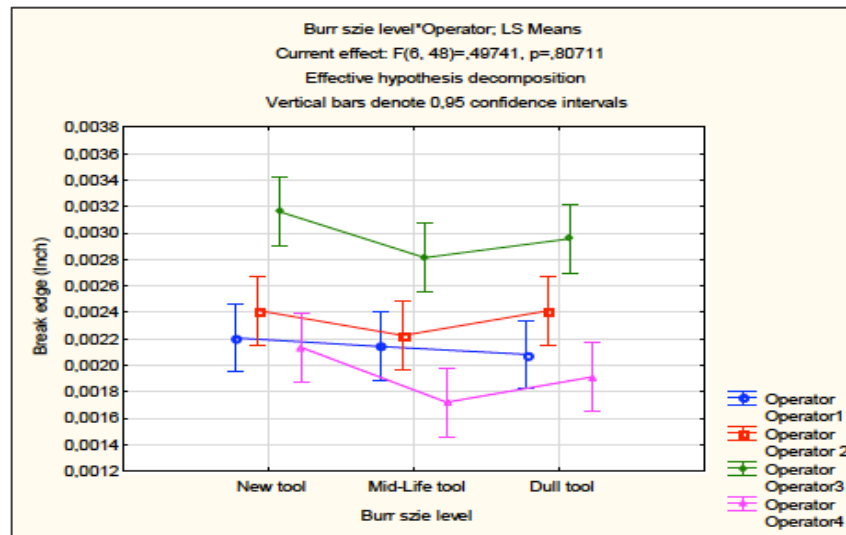
Figure 6-20 : Effect of burr size and operator on break edge (Part B)
