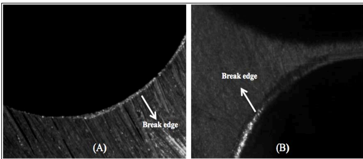
Figure 6-4: Wavy break edge created after filing (A), Enlarged and smooth break edge after buffing (B)
