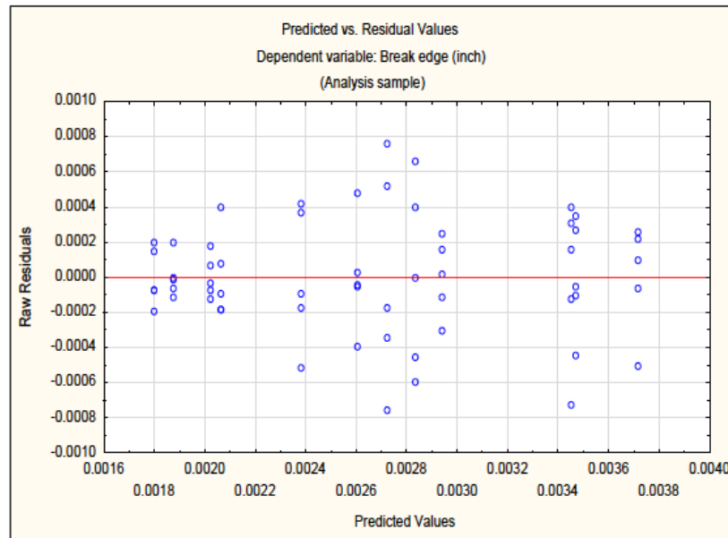
Figure 6-10: Residuals vs. predicted values (Part A)
