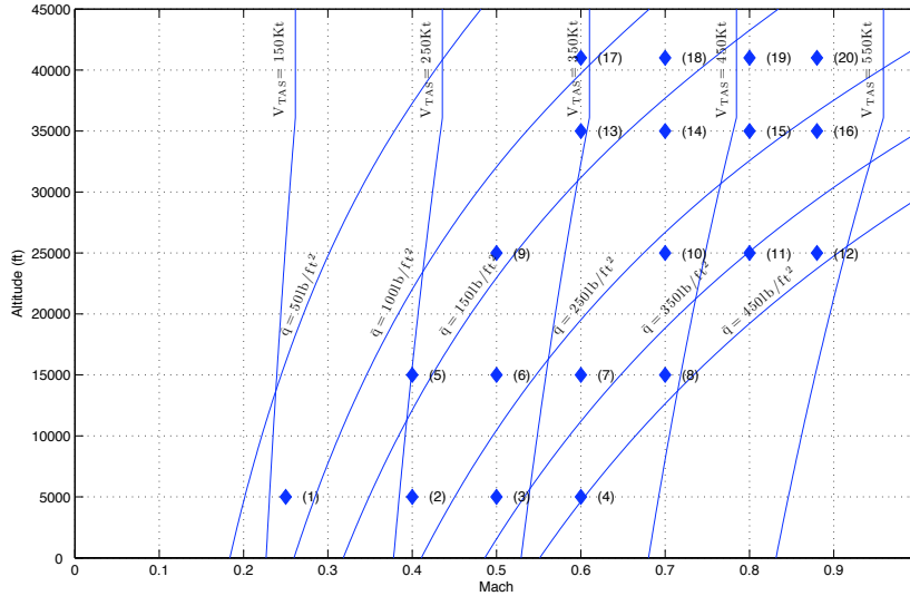
Figure 8.1 Flight envelope
