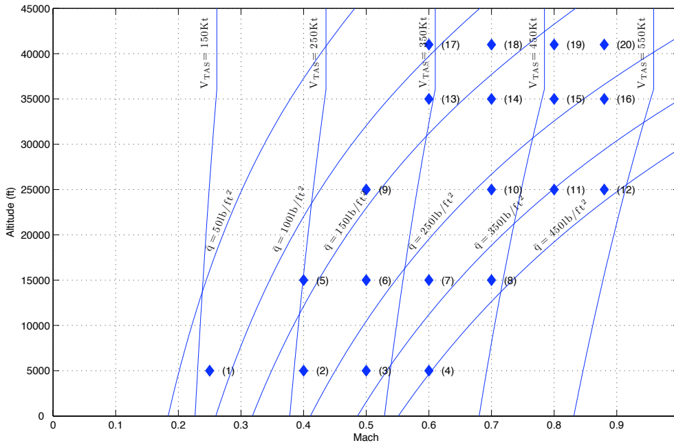
Figure 2.9 Enveloppe de vol
