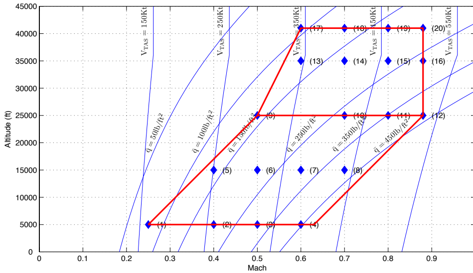
Figure 6.13 Flight envelope
