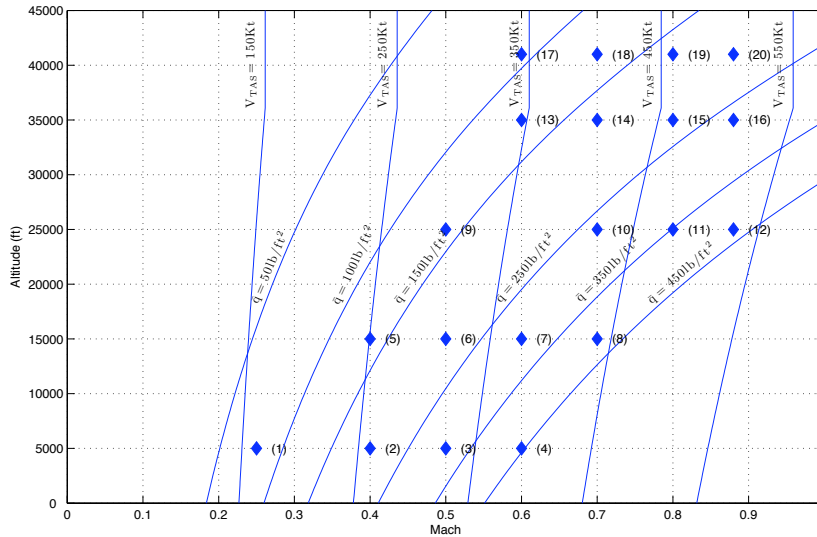
Figure 5.11 Flight envelope
