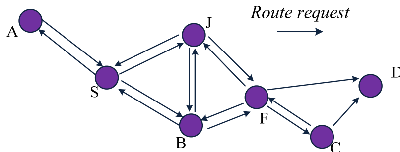
Figure 3.1: Flooding
