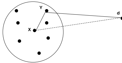
Figure 2.4: Greedy routing
