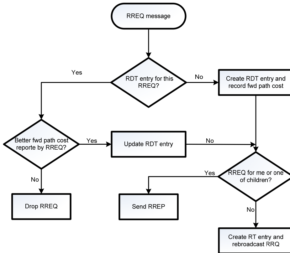
Figure 2.11: RREQ processing
