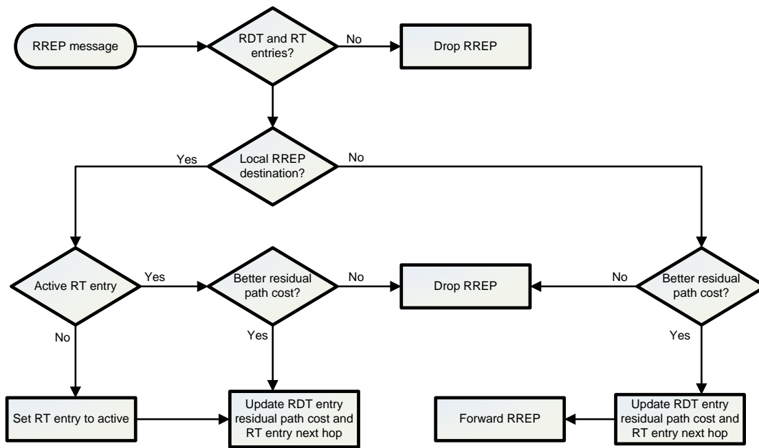
Figure 2.12: RREP processing
