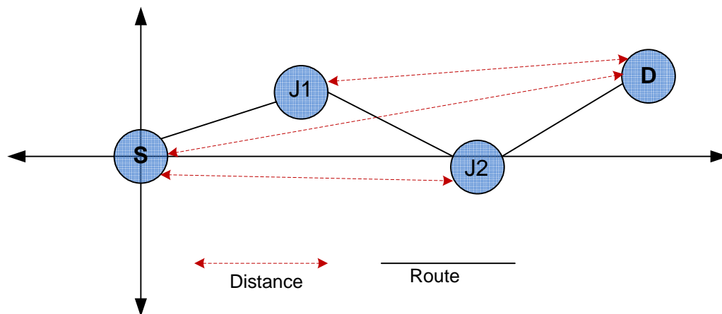
Figure 3.3: Location synchronization
