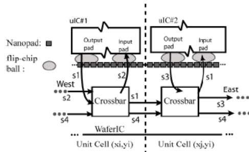
Figure 2: Routing example of a signal s_1 from a NanoPad in Unit Cell (x_i, y_i) redirected to another NanoPad of Unit Cell (x_j, y_j) towards the east. Signal s_4 passes through Unit Cells without interaction with the local uIC.
