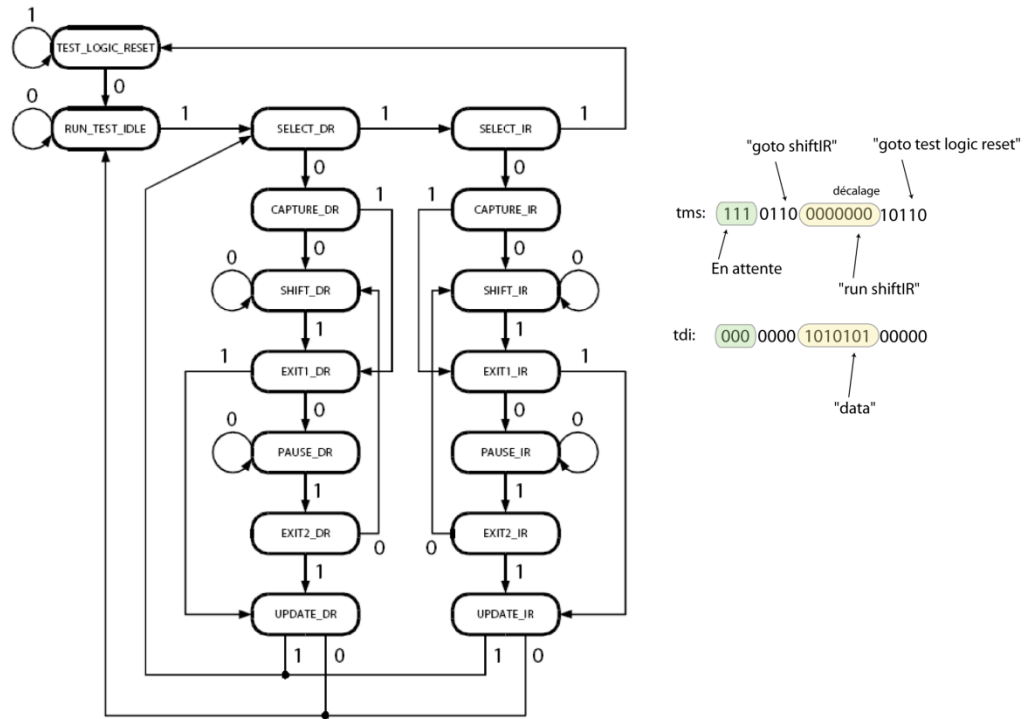
Figure 1: TAP State Machine Source: jtag.dev.java.net/
