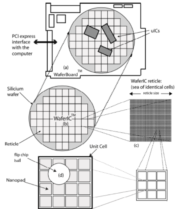
Figure 1: Illustration of the hierarchical structure of WaferBoard TM . (a) WaferBoard TM is connected to a computer via a PCI-express connection. (b) WaferIC TM is a sea of identical cells (c) residing on an external pc-board. The uIC/WaferIC TM contact is represented by a ball (d).
