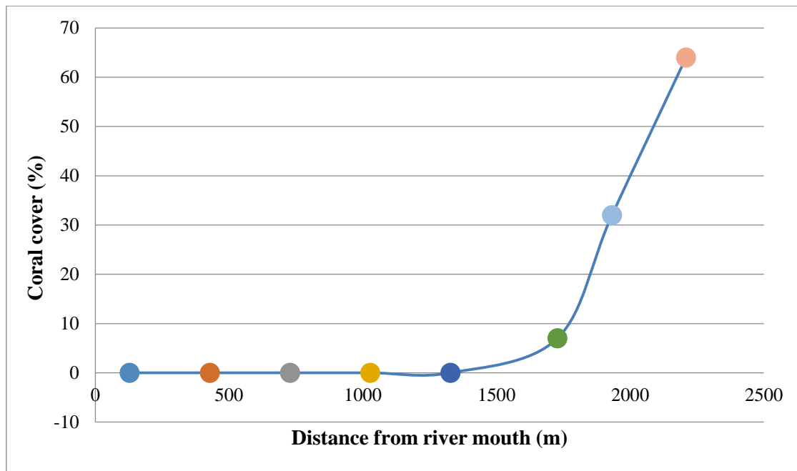
Figure 4.11: Coral distribution in Bonbon coastal waters showing a 1.6 km stretch of a river-associated coral-free zone, beyond which coral cover steeply increased.
