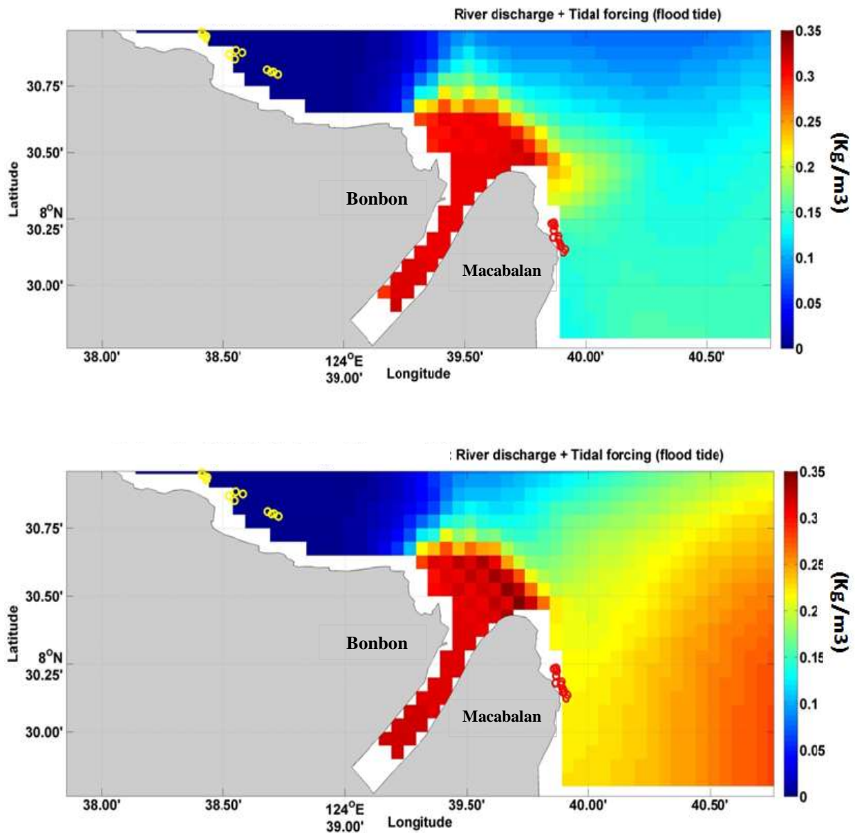
Figure 3.22: Influence of river discharge and tides on sediment plume at flood tide, both Layer 1 (top) and Layer 5 (bottom) resulted in an east and southeast net distribution of suspended sediment. The plume encroached on the seagrass site (red circles).
