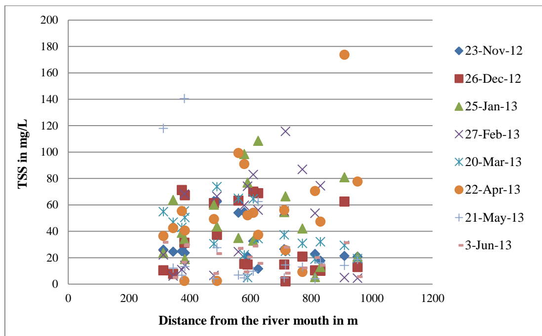
Figure 3.12: In Macabalan, no clear correlation between TSS values and distance from the river mouth was exhibited in any site. High-TSS concentration values (>20 mg/L) were distributed in all stations across the plot and so were low TSS values (<20 mg/L). Very high-TSS occurred as randomly distributed in several stations.
