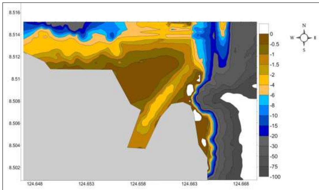
Figure 3.36: Bathymetric map of the coastal marine environments of the Cagayan de Oro River mouth, Macajalar Bay, showing relatively deep waters close to the Macabalan (east) coastlines and shallow waters in Bonbon (west); in particular, the mud accumulation along Bonbon shore. Units are in metres.
