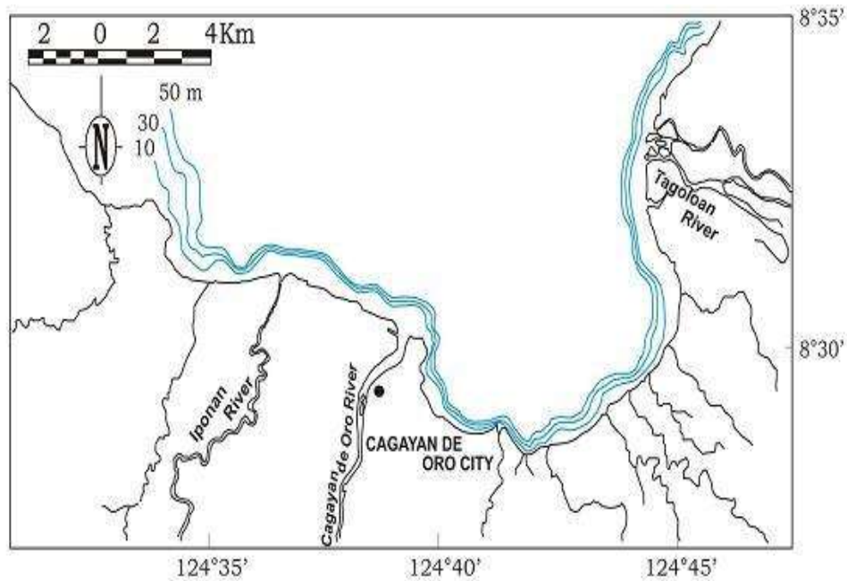
Figure 3.3: Macajalar Bay and the Cagayan de Oro River. Two major rivers, the Tagoloan and the Iponan, drain into the bay but are not included in the present study and modelling work. The bay is characteristically wide at its mouth and has a depressed curve on the southeast portion (source: NAMRIA map)
