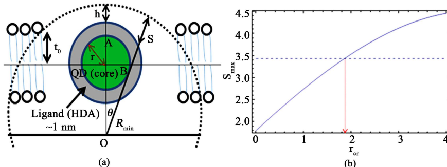
Figure 3. (a) A model representing the deformed monolayer due to the incorporation of a QD inside the lipid bilayer (b) A plot of chain length of the most stretched lipid, S_{\max} as a function of the QD radius, r ; The dotted line corresponds to the minimum radius R_{\min} of deformed lipid monolayer around QD.
