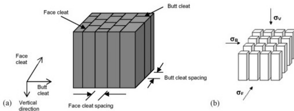
Figure 3.1 - Anisotropy of coal: (a) A coal fracture system; and (b) matchstick geometry showing anisotropic stresses (An et al., 2015)
