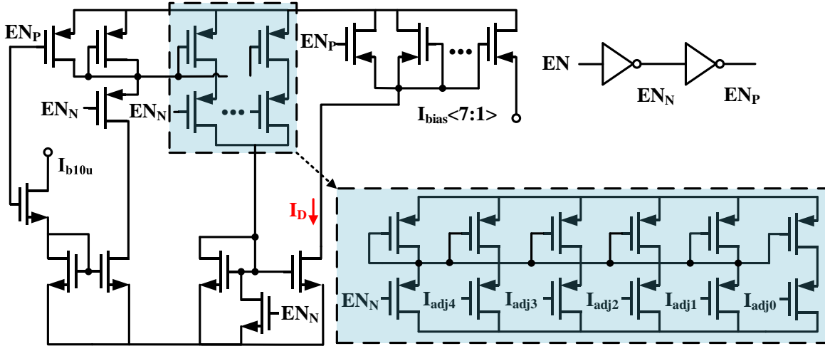
Fig. 10. Bias generator
