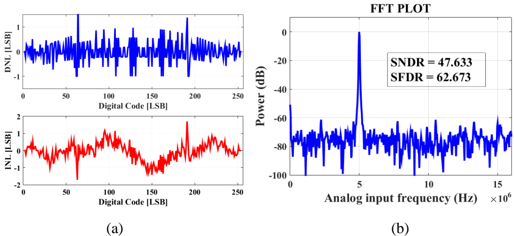
Fig. 14. Simulation results of DNL and INL, and FFT power plot
