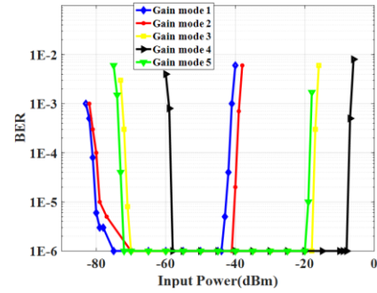
Fig. 8. Measured BER with five gain mode settings
