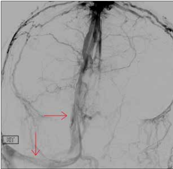
Figure 3. Coronal MRV contrast injection revealing improved drainage through superior sagittal sinus (horizontal arrow) and transverse sinus (vertical arrow) after venous sinus aspiration thrombectomy.
