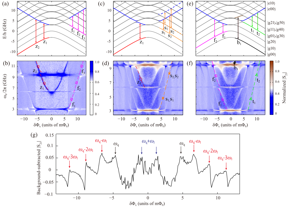
FIG. 2. [(a), (c), (e)] The energy levels of the coupled qubit-resonator system as a function of the flux bias \delta\Phi_x using parameters extracted from Fig. 1. The energy levels in the dispersive regime are labeled in terms of the uncoupled states |qN_1N_3\rangle . In panel (a), the red (magenta) arrows labeled as z_m ( f_m ) indicate the single-photon-driven zeroth-order qubit (first-order red-sideband) transition. In panel (c), the red (orange) arrows labeled as z_m ( s_m, s'_m ) indicate the single-photon-driven zeroth-order qubit (second-order red-sideband and cross-mode sideband) transition. In panel (e), the magenta (green) arrows labeled as f_m ( t_m ) indicate the single-photon-driven first-order (third-order) red-sideband transition and the black arrow labeled as b_1 indicates the single-photon-driven first-order blue-sideband transition. [(b), (d), (f)] The transmission (normalized |S_{21}| ) spectrum as a function of the flux bias \delta\Phi_x and driving frequency \omega_d/2\pi . In panel (b), for probe frequency of the 3\lambda/2 mode with probe power P_p \approx -132 dBm (average photon number n_3 \approx 0.19 ). The red-circle lines are due to the single-photon-driven zeroth-order qubit transition |g00\rangle \leftrightarrow |e00\rangle , corresponding to the red arrows in panel (a). The magenta-square lines are due to the single-photon-driven first-order red-sideband transition |g01\rangle \leftrightarrow |e00\rangle , corresponding to the magenta arrows in panel (a). [(d),(f)] Probe frequency of the \lambda/2 mode with probe power P_p \approx -128 dBm (average photon number n_1 \approx 11.7 ). In panel (d), the red-circle (orange-cross) lines are due to the single-photon-driven zeroth-order qubit (second-order red-sideband and cross-mode sideband) transition. In panel (f), the magenta-square (green-triangle) lines are the single-photon-driven first-order (third-order) red-sideband transition and the black-cross denoted short line indicates the single-photon-driven first-order blue-sideband transition. The power of the driving field on the resonator is P_d \approx -92 dBm for panel (b) and P_d \approx -97 dBm for panels (d) and (f). The effective field to drive the flux qubit is much reduced in the dispersive regime of the qubit-resonator system and the resulting average photon number in the resonator is far less than one (see Fig. 6 in Appendix B). (g) A linecut of the background-subtracted transmission spectrum in panel (d) at \omega_d/2\pi = 9.78 GHz, where the first-order blue sideband transitions purely due to the counter-rotating terms are marked with the blue arrows.
