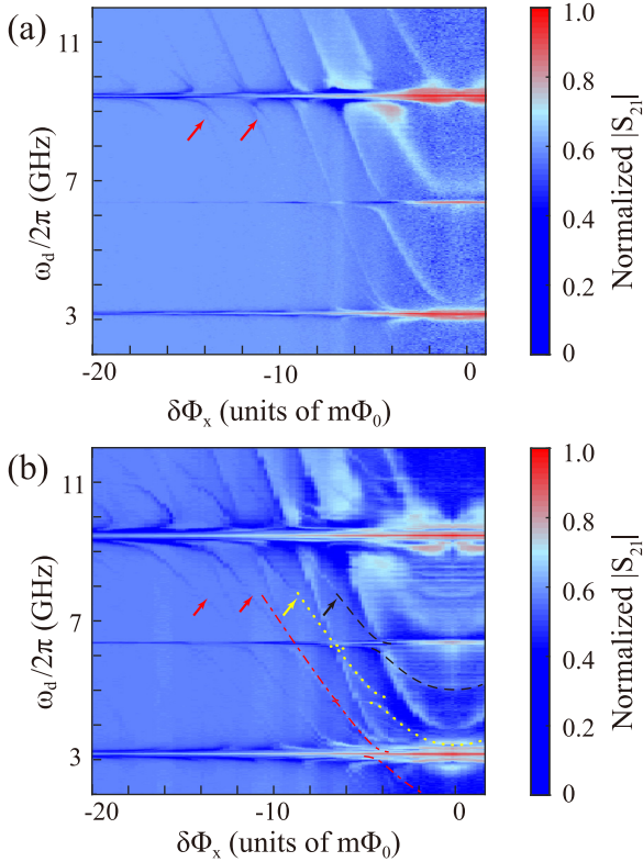
FIG. 3. The transmission spectroscopy (normalized |S_{21}| ) as a function of the flux bias \delta\Phi_x , and driving frequency \omega_d/2\pi probed at the frequency of \lambda/2 mode with power of P_p \approx -133 dBm, which contributes an average photon number n_1 \approx 3.34 into the resonator. With the driving power increased to (a) P_d \approx -92 dBm and (b) P_d \approx -82 dBm, the two-photon-driven sideband transitions ( 2\omega_d = \omega_q \pm s\omega_1 ) become visible, as indicated by the yellow arrows for the two-photon qubit transitions with s = 0 , the red arrows for the two-photon first- and second-order red-sideband transitions, and the black arrows for the two-photon first-order blue-sideband transitions. For clarity, here we only show in Fig. 3(b) the numerical fitting of the two-photon-driven first-order sideband transitions as labeled by the yellow, red, and black curves for 2\omega_d = \omega_q , 2\omega_d = \omega_q - \omega_1 , and 2\omega_d = \omega_q + \omega_1 , respectively.
