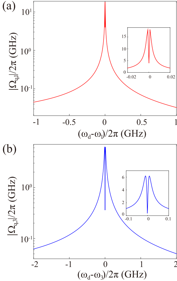
FIG. 5. Rabi frequency of the driving field on the flux qubit for (a) the \lambda/2 mode and (b) 3\lambda/2 mode. Each inset is a close-up of the near-resonance region between the driving field and the corresponding mode.
