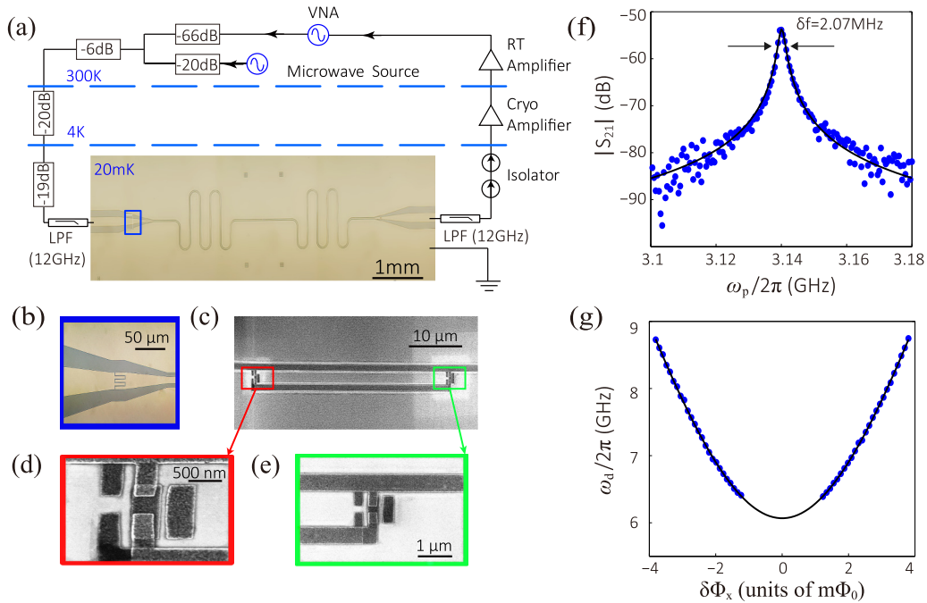
FIG. 4. (a) Optical image of the superconducting \lambda/2 coplanar waveguide resonator and schematic representation of the experimental setup. The transmission through the cavity at frequency \omega_p is measured using a vector network analyser (VNA). A second microwave signal at frequency \omega_d is used for qubit spectroscopy measurement. The input signal is attenuated and filtered at various temperature stages and coupled into the resonator through the capacitor. Two isolators and low-pass filters (LPF) are used to protect the sample from the cryoamplifier's noise. (b) Optical image of one of the two identical coupling capacitors of the resonator, as indicated by the blue rectangle area in panel (a). (c) Scanning electron microscope (SEM) image of the galvanically connected flux loop (the red and green rectangular areas are shown in panels (d) and (e), respectively). The shared arm between the flux qubit and the resonator's center line is 34.8 \mu\text{m} long and 800 nm wide. (d) SEM image of the left two Josephson junctions in the flux qubit loop. (e) SEM image of the right two Josephson junctions in the flux qubit loop. (f) Transmission spectra of the \lambda/2 resonator mode, which is measured at 20 mK. The black continuous line shows the Lorentzian fit to the transmission power spectrum. The resonance frequency \omega_1/2\pi = 3.143 GHz and FWHM of 2.07 MHz are obtained by the fitting. (g) Qubit transition frequency \omega_q from spectroscopy measurement vs relative magnetic flux bias \delta\Phi_x . The data are recorded at a probe power P_p \approx -143 dBm (corresponding to an average photon number n_1 \approx 0.19 in the resonator). The probe frequency is equal to the frequency of the \lambda/2 mode. The black continuous line represents a numerical fit to the qubit Hamiltonian H_q yielding the parameters \delta/h = 6 GHz and I_p = 265 nA.
