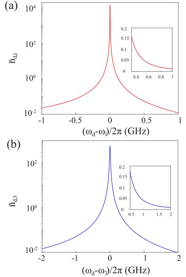
FIG. 6. Average number of photons in the resonator that come from the driving field. (a) \lambda/2 mode and (b) 3\lambda/2 mode. Each inset is a zoom of the off-resonance region between the driving field and the corresponding mode.
