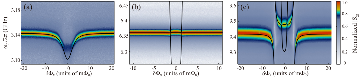
FIG. 1. (a) The transmission (i.e., the normalized |S_{21}| ) spectrum of the \lambda/2 mode as a function of the flux bias \delta\Phi_x and probe frequency \omega_p/2\pi . The probe power is P_p \approx -138 dBm, corresponding to an average photon number of n_1 \approx 1.17 in the resonator. (b) The spectrum of the \lambda mode with P_p \approx -135 dBm and average photon number n_2 \approx 0.24 . (c) The spectrum of the 3\lambda/2 mode with P_p \approx -132 dBm and average photon number n_3 \approx 0.19 . The solid curves are the numerical fits of the spectra with respect to its ground-state energy using the full Hamiltonian H .
