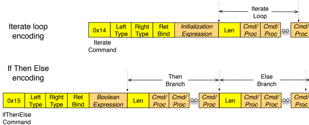
Figure 4.2: Protocol Packing of Conditionals
