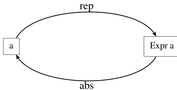
Figure 2.5: Expression Transformation
