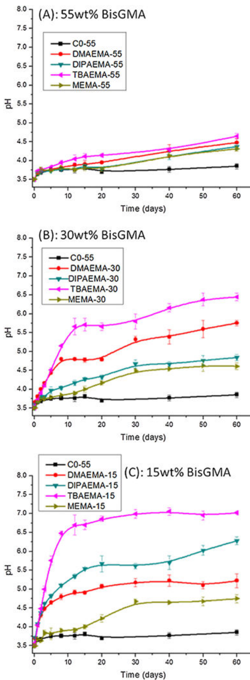
Fig. 1. Plots showing the ability of different amine-containing polymers to neutralize LA. Each plot shows the pH of a set of amine-containing polymers with equivalent BisGMA concentration as a function of incubation time. (A) 55 wt% BisGMA; (B) 30 wt% BisGMA; (C) 15 wt% BisGMA. The control formulation (C0-55), which lacks amine moieties, is shown in black on each plot for comparison.
