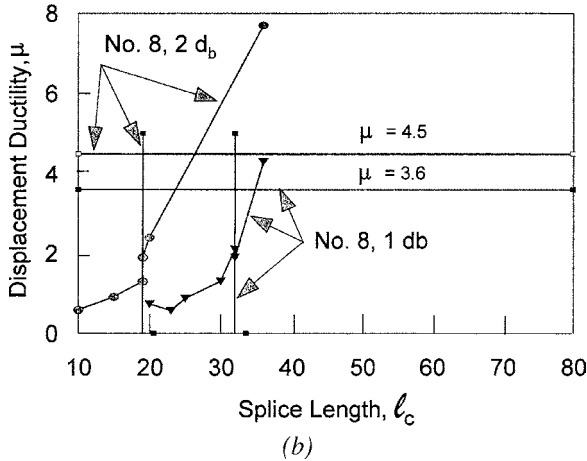
Fig. 3—Displacement ductility versus splice length for: (a) No. 11 (No. 36) bars; and (b) No. 8 (No. 25) bars.
