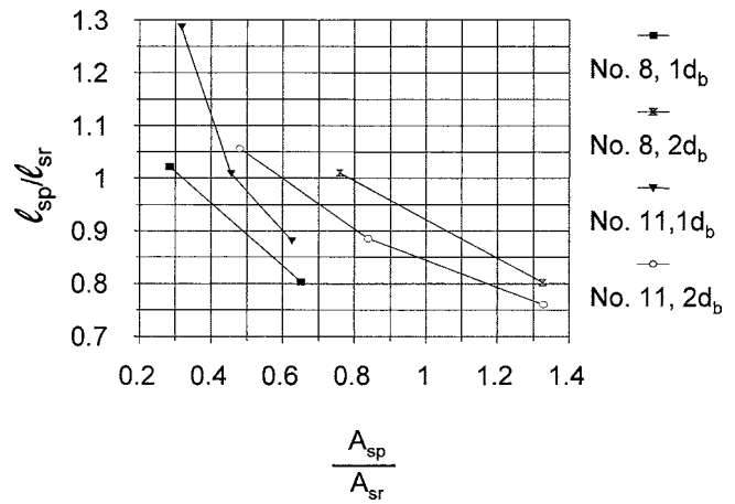
Fig. 8—Ratio of development provided l_{sp} to development length required by ACI 318-95 without transverse reinforcement and within no limit on \sqrt{f'_c} , l_{sr} versus A_{sp}/A_{sr} .
