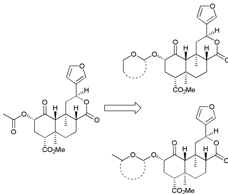
Figure 1. Eclipsed (upper) or extended (lower) conformations of the ethoxymethyl ether at C-2 compared to salvinorin A.
