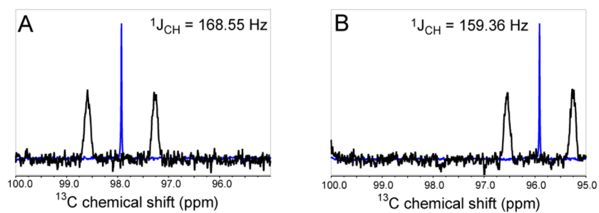
Figure 2. 1D ^{13}\text{C} NMR spectrum with composite pulse ^1\text{H} -decoupling (blue) and gated decoupling to show J_{\text{C,H}} (black) for the anomeric carbon of 5 (A) and 6 (B).
