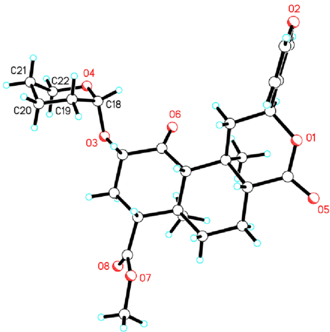
Figure 3. X-ray crystallographic structure of 5 .
