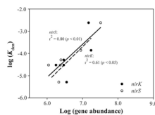
Fig. 2. Relationship between log-transformed nirS - (○) and nirK - (●) gene abundances and log-transformed denitrification coefficient ( K_{den} ). Note: Values for Shane Creek were excluded from the graph due to the inability to log-transform the K_{den} value ( K_{den} = .0 \text{ m}^{-1} ). nirS and nirK were 10^{6.2} and 10^{6.1} genes per g-dry sediment for this stream.
