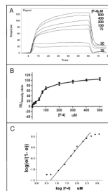
Figure Seven. Surface Plasmon Resonance (SPR) Analysis of F-4 Binding Hsp90 SPR analysis of the binding of F-4 to Hsp90 was carried out as described under Materials and Methods . Panel A demonstrates representative binding curves of F-4 injected at the indicated concentrations, while panel B displays replot of relative units at steady state (RU steadystate : amount bound) versus concentration of F-4. Panel C displays a Hill plot of the binding of F-4 to Hsp90.
