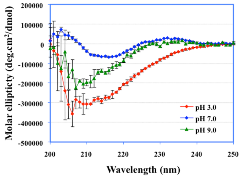
Fig. 2. The CD spectra of EC1-IN in buffered solutions at pH 3.0, 7.0, and 9.0. The secondary structure of EC1-IN is affected by the pH of the solution.
