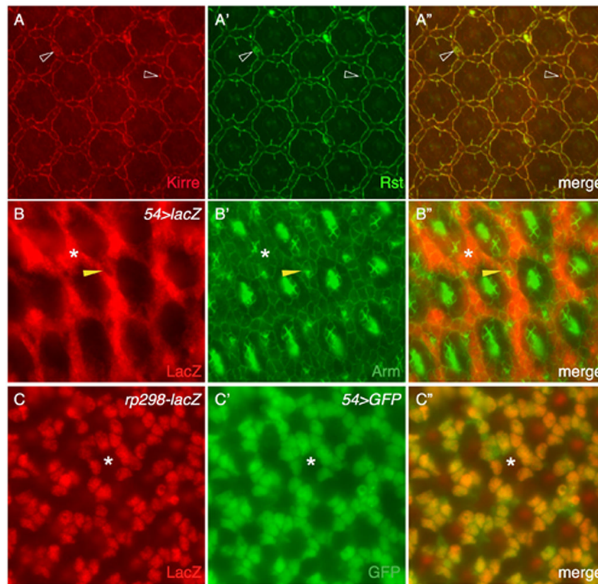
Figure 2. Kirre is expressed in IOCs. (A-A'') Kirre (red) co-localizes with Rst (green) on the surface. Kirre also co-localizes with Rst in all vesicles (open arrowheads). (B-B'') The Gal4-54; UAS-lacZ (54>lacZ) eye at 27 h APF was co-stained with anti-lacZ (red, left) and anti-Armadillo (green, middle) antibodies. Merged view is shown in the right panel. LacZ was detected exclusively in IOCs (asterisks). Arrowheads point to a bristle group from which lacZ staining was absent. (C-C'') kirre is transcribed in IOCs as revealed by an enhancer trap rp298-lacZ . The eye was stained with an anti-LacZ antibody (red) and marked by 54>GFP (green). Space for an ommatidium is indicated by an asterisk.
