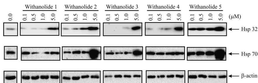
Figure 2. Western blot analysis of glioblastoma cell line U251 following treatment with withanolides 1–5. Total levels of HSP32 and HSP70, biomarkers of cellular stress and withanolide activity, were screened at 0, 0.1, 0.5, 1, and 5 μM concentrations of each compound for 24 h. HSP70 was markedly upregulated at 5 μM with withanolides 2, 3, and 5, while HSP32 levels were elevated in a concentration-dependent manner with all compounds 1–5 tested. The β-actin protein was used as a loading control marker.
