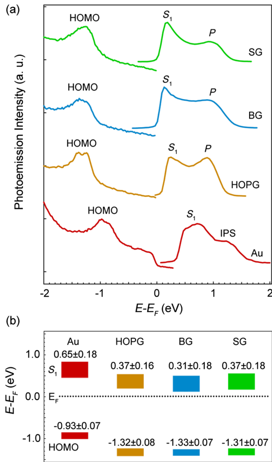
FIG. 2 Energy-level alignment at the interface. (a) UPS (left) and 2PPE (right) spectra for 0.5 nm ZnPc films deposited on various surfaces, which show the occupied and unoccupied band structures, respectively. The energy is referenced with respect to the Fermi level E_F . (SG, single-layer graphene; BG, bilayer graphene; HOPG, graphite; and Au, gold.) (b) The alignment of the HOMO (bottom) and S_1 state (top) of ZnPc with respect to E_F . The unit for the numbers is eV.
