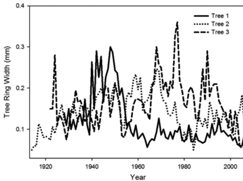
Fig. 1. Tree ring growth series with raw ring width (mm) plotted across time. Data presented are representative of a random sample of tree rings from the tree populations described in the text.
