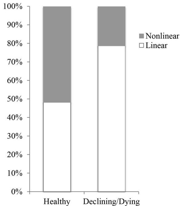
Fig. 3. S-map-classified dynamics from healthy and declining or dying trees from red oaks in Arkansas, USA. Healthy trees were significantly more likely to have nonlinear dynamics ( p = 0.015 ). Analysis shown here combines declining and dying trees into one unhealthy class.
