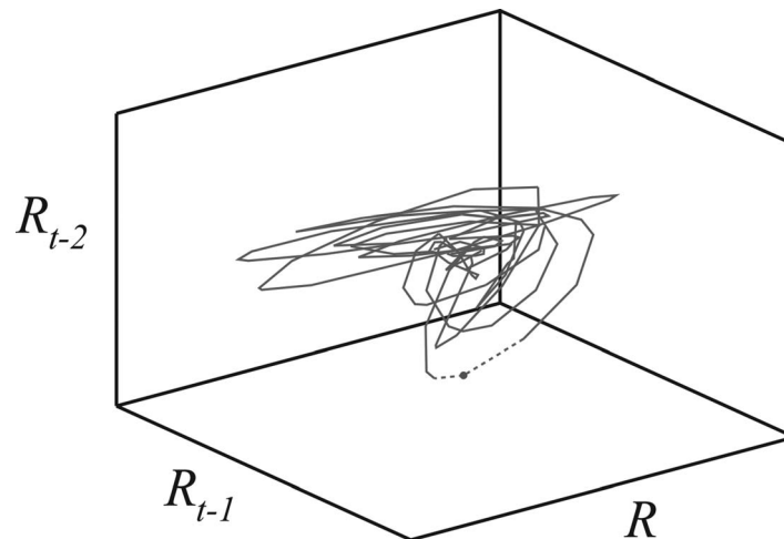
Fig. 2. Hypothetical example of a lagged coordinate embedding used to reconstruct system dynamics (state space reconstruction) to facilitate simplex projection and S-map modeling. The model, an attractor, is constructed by plotting consecutive lags at various time steps ( t ) ( R_t , R_{t-1} , R_{t-2} ) of the system variable in question (here, tree radial growth represented by R ). The number of axes (and therefore number of time lags used) equals the embedding dimension, E , of the state space. Each coordinate in the attractor is therefore a vector of length E that is used to create library and prediction vectors for our two forecasting models. In our approach, the model is built from a set of library vectors (joined by solid lines) used to forecast one prediction vector (the dot, located along the dashed line).
