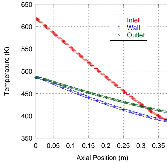
Figure 76: Temperature profiles of neighboring inlet channel, wall, and outlet channel
