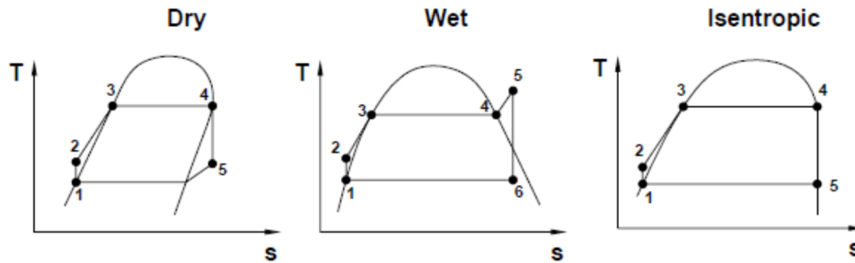
Figure 7: Classification of working fluids by saturated vapor curve slope [51] (Reprinted with Permission from SAE International)
