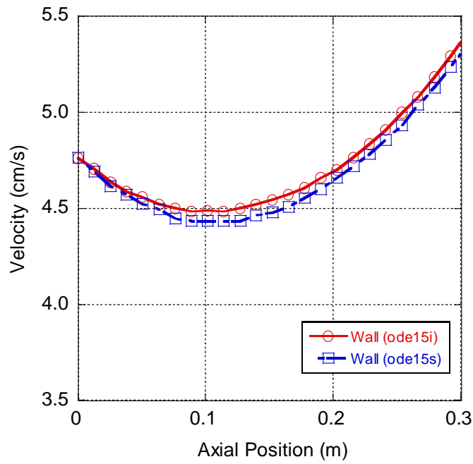
Figure 36: Wall velocity profiles for model comparison
