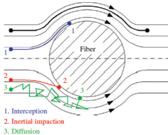
Figure 26: Methods of particle collection by a single fiber [97] (Reprinted with Permission from SAE International)
