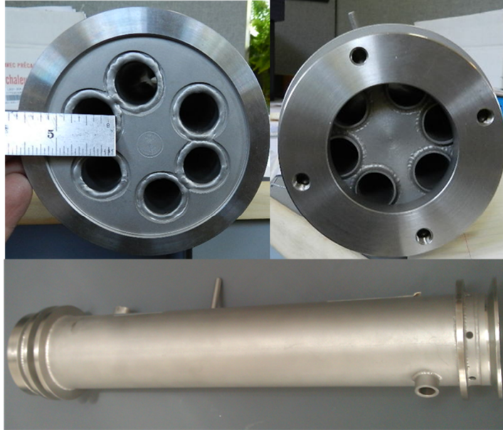
Figure 53: End and side views of heat exchanger for WHR experiments
