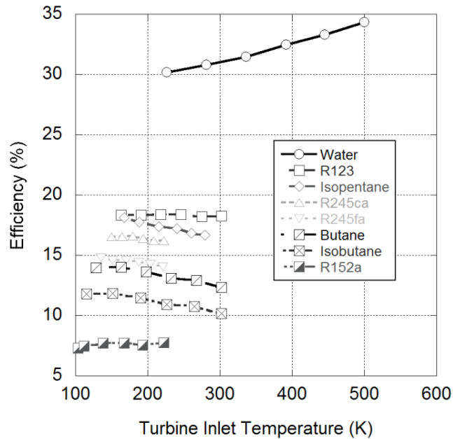
Figure 14: Rankine cycle efficiency for various working fluids [51] (Reprinted with Permission from SAE International)
