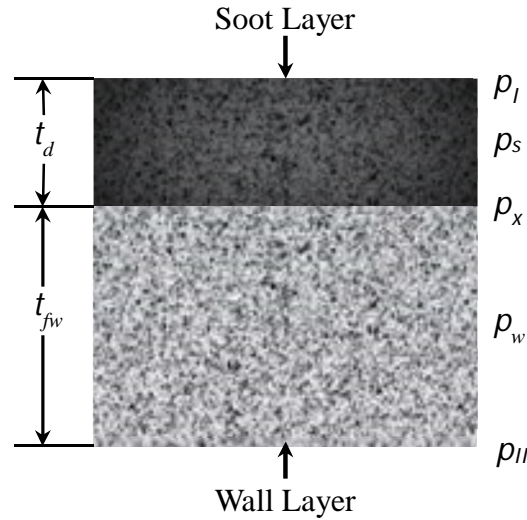
Figure 30: Schematic of two wall velocity pressures through soot and wall layers
