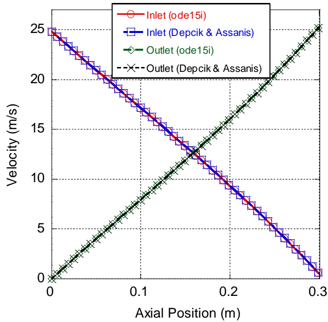
Figure 39: Velocity comparison with literature values
