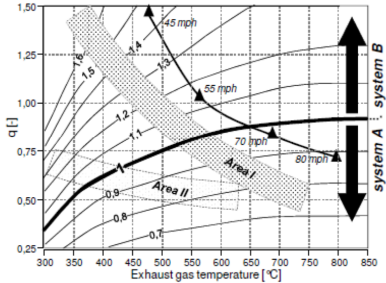
Figure 16: Comparison of system performance with vehicle speed [17] (Reprinted with Permission from SAE International)
