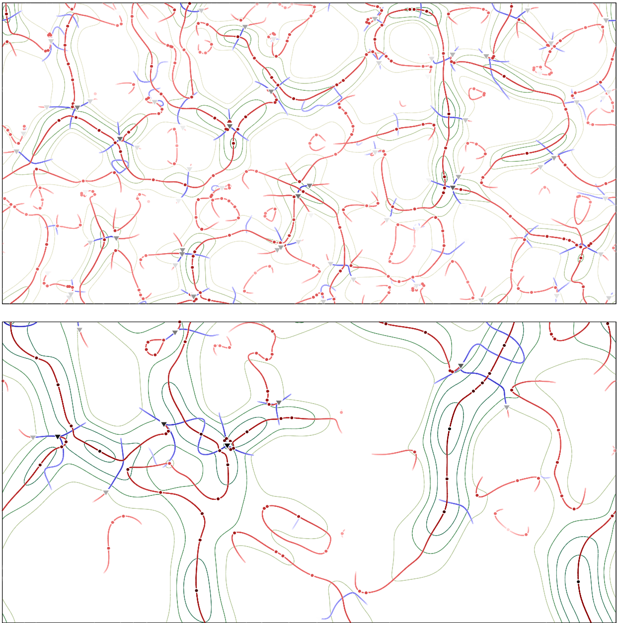
Figure 17. Singularity structure as function of power spectrum. A_3 lines for two different power spectra, P(k) = k^k , k = 4 (top), k = -1 (bottom) both smoothed at the same scale. As expected for power spectra with a positive index, the pattern is much more regular. What is even more interesting is that the clustering statistics of the singularities seem to change in a non-trivial way. This will be the topic of a follow-up paper.
