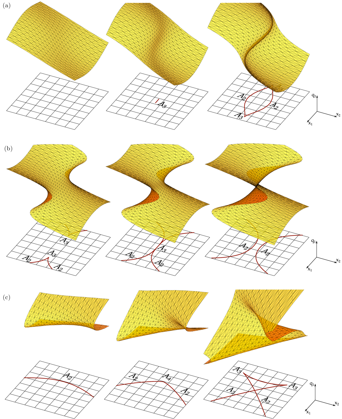
Figure 3. A-series of singularities. The figures shows the 3D projection of the Euler–Lagrange phase-space sheet on to the configuration space (x_1, x_2, q_1) , with q_1 along the vertical direction and the Eulerian plane (x_1, x_2) in the horizontal direction. The smooth yellow surface is the 3D projection of the phase-space sheet. Each singularity is shown at three different time steps. Each image shows the phase-space sheet at one particular instant, along with the caustic structure – the black solid lines – in the 2D projection on the Eulerian (x_1, x_2) plane. Although the images are rather schematic, these illustrations are fully representative for the general case that we encounter in the evolving cosmic mass distribution. (a) A_3^+ , the birth of a pancake. The linear term in the surface counters the cubic term, generating the singularity when the magnitude of their derivatives matches. This linear term grows with time, faster in the middle. (b) A_3^- singularity and the merging of two pancakes. The linear term in surface has a minimum in the middle. So this is where the surface tangent goes singular last, joining the two three-stream regions that are already present. (c) The A_4 swallow-tail singularity and the folding of a pancake. In the first image, we see the edge of a pancake. This pancake develops a singularity, that then unfolds into two cusps moving away from each other.
