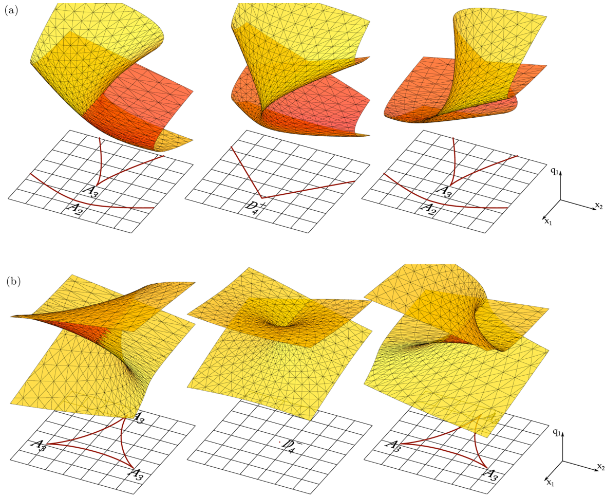
Figure 4. The D -series of singularities, limited to the D_4 singularities. The figures shows the 3D projection of the Euler–Lagrange phase-space sheet on to the configuration space (x_1, x_2, q_1) , with q_1 along the vertical direction and the Eulerian plane (x_1, x_2) in the horizontal direction. The smooth yellow surface is the 3D projection of the phase-space sheet. Each singularity is shown at three different time steps. Each image shows the phase-space sheet at one particular instant, along with the caustic structure – in the 2D projection on the Eulerian (x_1, x_2) plane. Although the images are rather schematic, these illustrations are fully representative for the general case that we encounter in the evolving cosmic mass distribution. (a) The D_4^+ singularity: the hyperbolic umbilic. The structure of this singularity cannot be embedded in 3D without having self-intersecting surfaces. Note that the centre image shows a symmetric surface, but the deprojection of it resembles an earlier (or later) stage of development. The projection of two folds coincides. This will always happen locally at a D_4^+ point. Thom (1969) called this singularity a ‘purse’. (b) The D_4^- singularity: the elliptic umbilic. This singularity produces the steepest density profile possible in 2D. Thom (1969) called this singularity a ‘pyramid’.
