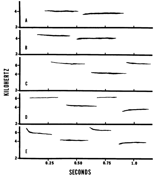
Fig. 3. Tracings of spectrograms of Missouri chickadee vocalizations. KiloHertz scale is logarithmic. (A) P. atricapillus song from Site 1. (B–D) Two-noted, three-noted, and four-noted songs of a single contact zone individual from Site 3. (E) P. carolinensis song from Site 4.
