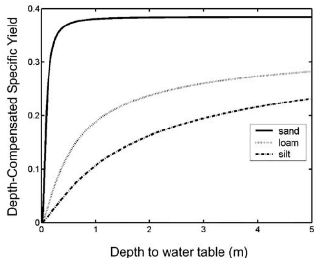
Figure 7. Depth-compensated specific yield as a function of depth to the water table for sand, loam, and silt textures. Specific yield calculated as θ S - θ R is 0.385, 0.352, and 0.426 for the sand, loam, and silt textures, respectively.
