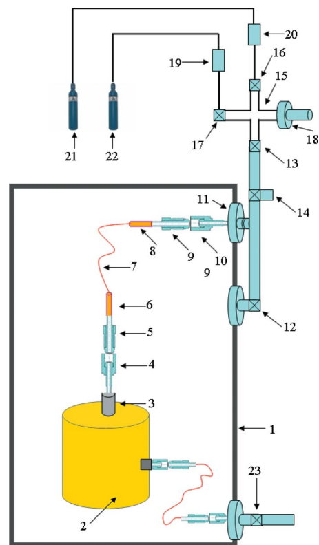
FIG. 4. (Color online) Scheme showing the introduction of high pressure reactant gases to reactor when the reactor is under UHV environment of the STM chamber. (1) STM chamber, (2) high pressure reactor, (3) stainless steel tube (inside diameter= \frac{1}{8} in.), [(4) and (10)] male part of a Swagelok fitting, [(5) and (9)] female part of a Swagelok fitting, [(6) and (8)] silica-coated stainless steel tube (inside diameter= \frac{1}{16} in.), (7) PEEK tubing (outside diameter= \frac{1}{16} in., inside diameter= \frac{1}{32} in.), (11) double side CF flange, [(12) and (13)] angle valves, (14) angle valve for pumping reactant gases after completion of a batch mode high pressure experiments, (15) vessel for mixing different reactant gases, [(16) and (17)] variable leak valves, (18) Baratron capacitance manometer for pressure measurements, [(19) and (20)] gas filters, [(21) and (22)] gas cylinders, and (23) angle valve.
