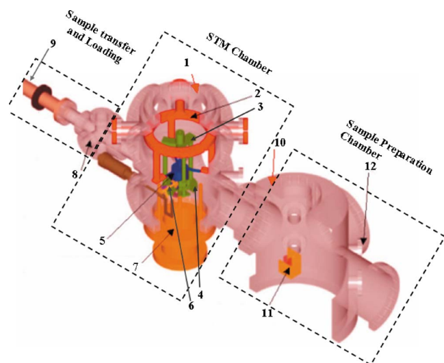
FIG. 1. (Color online) Schematic of STM and UHV systems: (1) view window, (2) mounting framework, (3) docking scaffold, (4) docking disk, (5) high pressure reactor (STM body housed within), (6) bayonet seal, (7) guide rod of docking scaffold, (8) sample/tip load-lock system, (9) transfer rod, (10) gate valve, (11) four-finger sample stage, and (12) sputtering ion gun.
