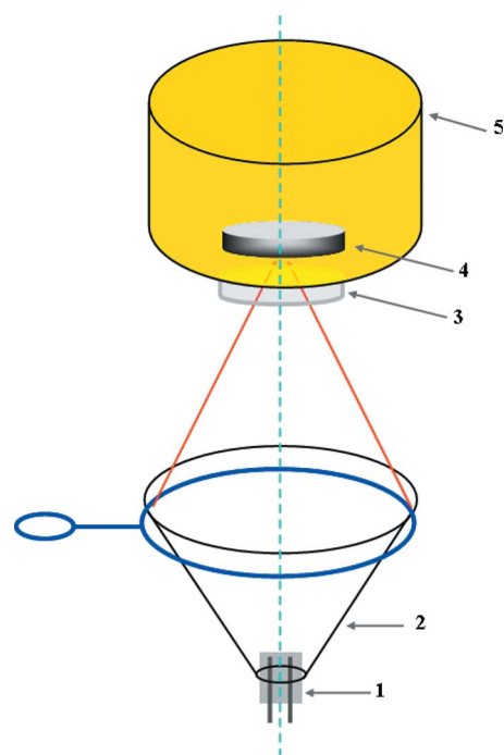
FIG. 2. (Color online) STM chamber in situ sample heating system: (1) halogen lamp, (2) elliptical reflector, (3) sapphire window welded at the center of the bottom of the high pressure reactor, and (4) the assembled sample, (5) high pressure reactor. The turquoise dashed line shows the alignment of light beam and sample center.
