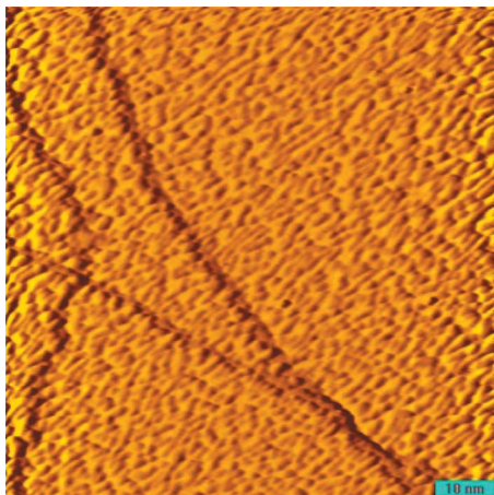
FIG. 8. (Color online) STM image of a highly roughed Pt(100) formed in an environment of 0.9 bar CO.
