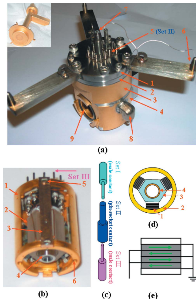
FIG. 3. (Color online) High pressure reactor and STM body. (a) A view of the whole reactor: (1) cell lid, (2) cell neck, (3) middle stage, (4) bottom stage, (5) pin-socket contacts for wiring of STM body at the interface of high vacuum and high pressure environment, (6) a pin on the lever of the cell lid for mounting, (7) Swagelok fitting welded on the tube of the cell lid for gas introduction, (8) Swagelok fitting welded on the button stage of reactor for sample and tip transfer. (b) Side view of the STM body: (1) wall of STM body coated with a layer of gold, (2) hexagonal sapphire, (3) CuBe spring plates, (4) receiver of tip holder, (5) screw to adjust the pressure applied to hexagonal sapphire, and (6) hole to assemble sample stage to STM body. (c) Scheme of pin-socket alignment for wiring. Set III is the contacts glued to the holes on top of STM body; set II is the contacts glued to the holes on top of cell lid of the reactor; set I is the contacts glued to wires from docking scaffold. (d) Scheme showing the assembly of three packs of shear piezoelectric plates between the hexagonal sapphire and the wall of the STM body and the assembly of the scanning tube: (1) a set of piezoelectric plates, (2) wall of STM body, (3) hexagonal sapphire, and (4) scanning tube. (e) Scheme showing how the four shear piezoelectric plates of one set work for coarse approach. Two alumina plates are glued to the first and fourth shear piezoelectric plates for thermal isolation and electrical insulation.
