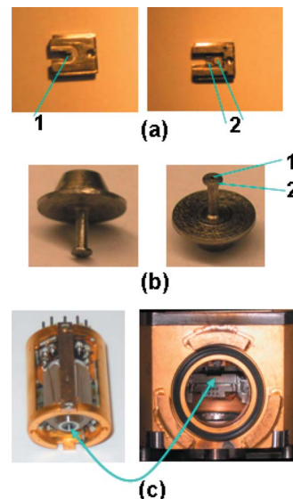
FIG. 5. (Color online) Parts used for a convenient tip exchange. (a) Tip exchanger; (1) the central slot which has a size between the stopping disk and outer diameter of the tube of the tip holder; (2) magnets. (b) Tip holder with an empty tube for placing a tip; (1) empty tube for placing a STM tip; (2) stopping disk. (c) Magnetic bowl glued at the end of the scanning tube. The arrow shows the hidden bowl at the end of the scanning tube.
