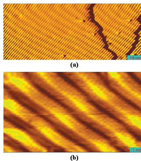
FIG. 7. (Color online) (a) Large-size STM image of a clean surface of hex-Pt(100) with step height of single atom collected under UHV condition at 300 K. (b) Small-size atom-resolved image of this surface under UHV.
