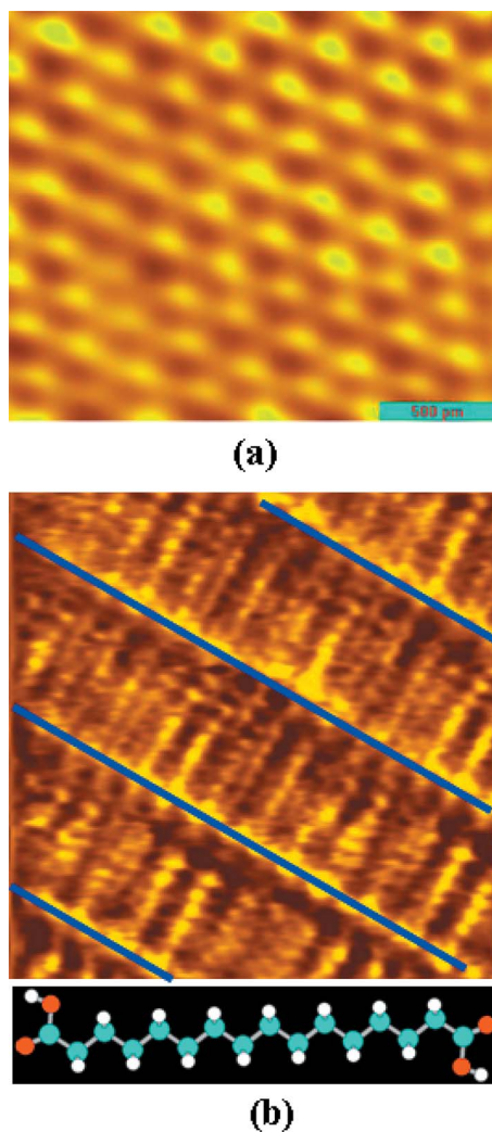
FIG. 6. (Color online) (a) STM image of a clean HOPG surface. (b) STM image of a self-assembled monolayer of hexadecanedioic acid deposited on HOPG under an environment of 1 bar nitrogen; the bottom is the structure of the molecules self-assembled on HOPG.
