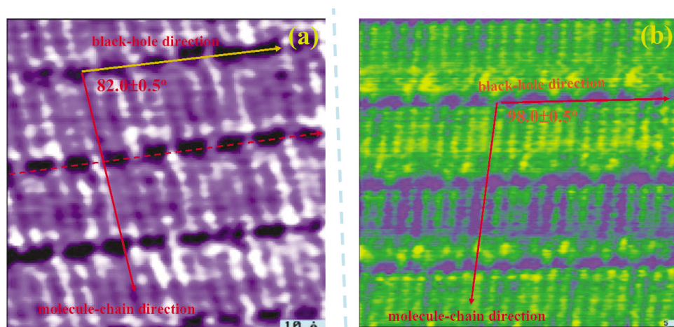
Fig. 7 Two kinds of domains ( m and m' ) formed by self-assembly of achiral arachidic anhydride. The dimensions in images (a) and (b) are 72 \times 72 \text{ \AA} and 93 \times 93 \text{ \AA} , respectively. The turquoise dashed line between images (a) and (b) is the mirror plane between the two enantiopure domains. Red dashed line shows the black-hole rows.
