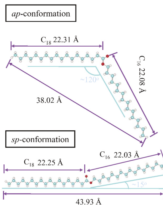
Fig. 4 ap and sp conformations of stearic acid palmityl ester molecules.
