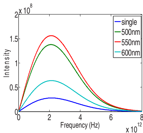
FIG. 14. (Color online) Terahertz radiation in the far field for nanoparticle ring structures (single nanoparticle ring, d=500 , 550 , and 600 nm, respectively).
