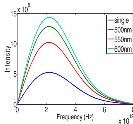
FIG. 13. (Color online) Terahertz radiation in the far field for nanoparticle structures (single nanoparticle, d=500 , 550, and 600 nm, respectively).
