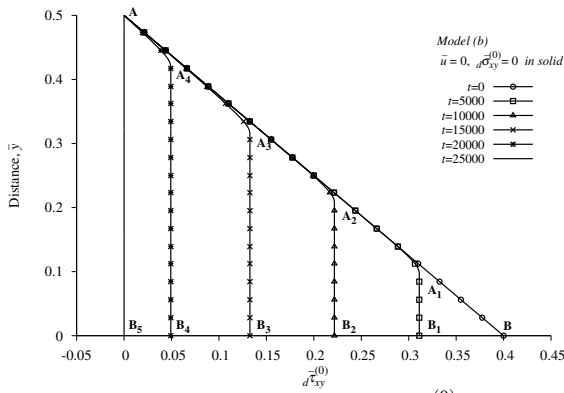
Figure 43: Model Problem 6: Evolution of {}_d\bar{\tau}_{xy}^{(0)} using model (b), C^{11}(\bar{\Omega}_{xt}^e) , p = 9, \Delta t = 50
