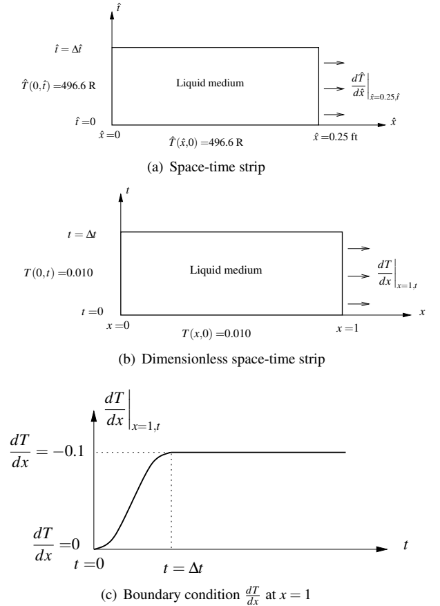
Figure 10: Liquid-solid phase transition: space-time strip, boundary conditions, and initial condition
