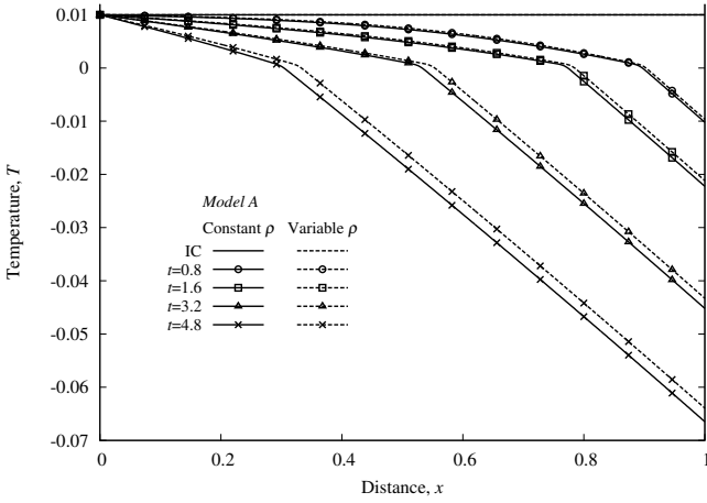
(b) Evolution of temperature, 0.0 \leq t \leq 4.8
