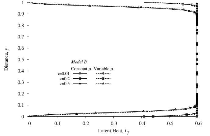
(a) Evolution of latent heat at the centerline
