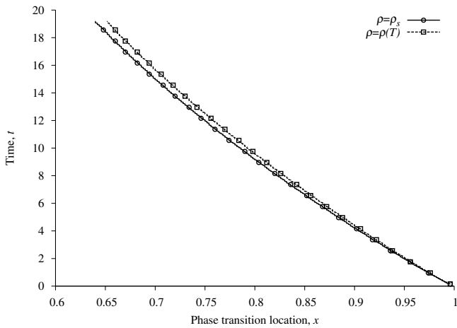
Figure 23: Model Problem 3: Interface location as a function of time, C^{11}(\bar{\Omega}_{\Delta t}^e) , p = 9, \Delta t = 0.04
