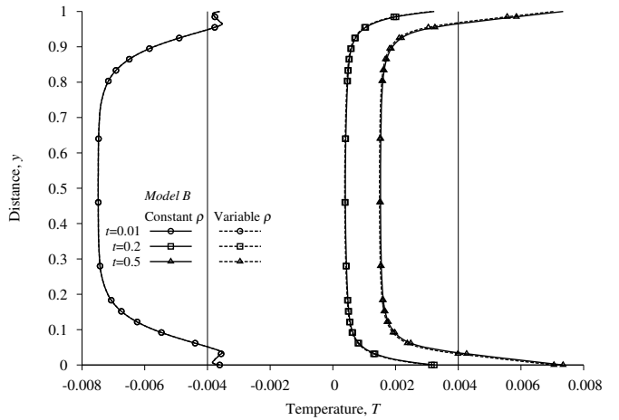
(b) Evolution of temperature at the boundary
