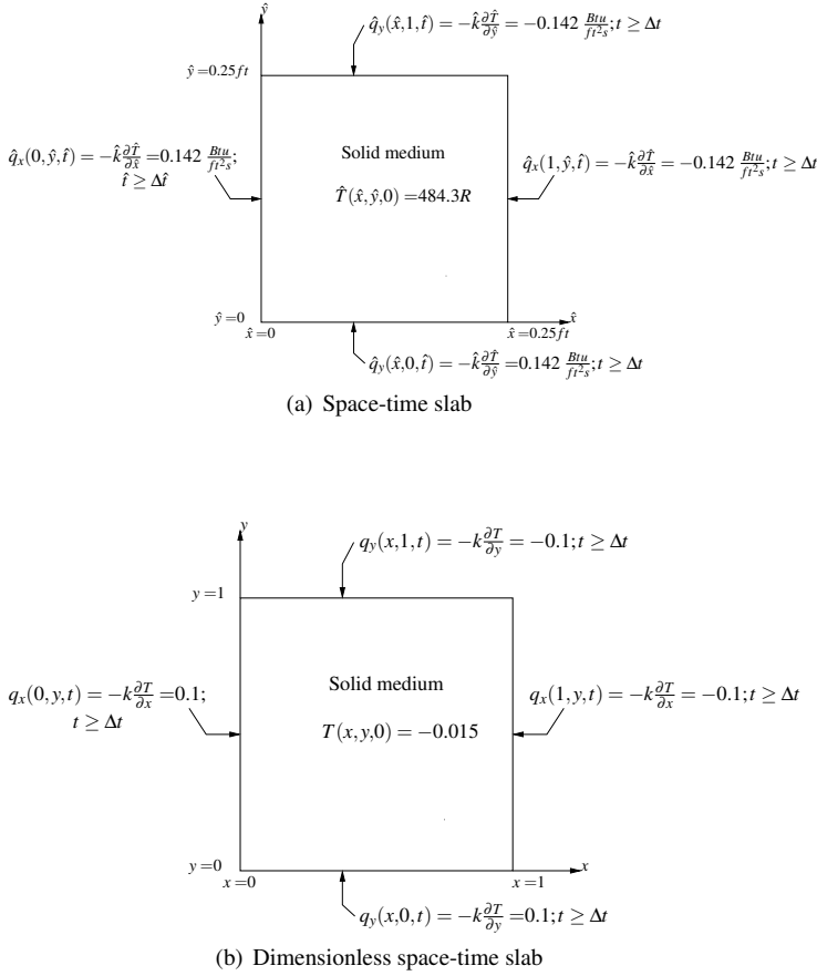
Figure 30: 2D solid-liquid phase transition: space-time slab, boundary conditions, and initial condition
