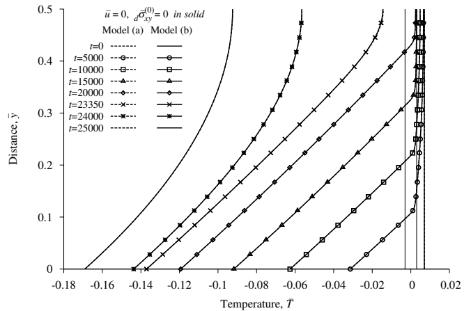
Figure 45: Model Problem 6: Evolution of temperature \bar{T} versus \bar{y} using model (a), C^{11}(\bar{\Omega}_{xt}^e) , p = 9, \Delta t = 50
