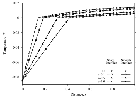
Figure 7: Model Problem 1: Evolution of temperature using smooth-interface model and sharp-interface theoretical solution, C^{11}(\bar{Q}_{st}^e) , p = 7 , \Delta t = 0.01
