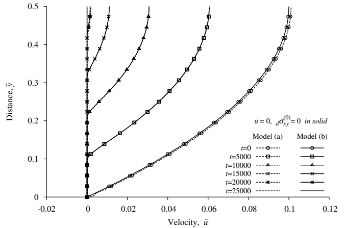
Figure 44: Model Problem 6: Evolution of velocity \bar{u} versus \bar{y} using model (a), C^{11}(\bar{\Omega}_{xt}^e) , p = 9, \Delta t = 50
