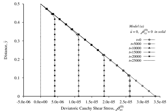
Figure 46: Model Problem 6: Evolution of deviatoric Cauchy shear stress {}_d\bar{\sigma}_{xy}^{(0)} using model (a), C^{11}(\bar{\Omega}_{xt}^e) , p = 9, \Delta t = 50
