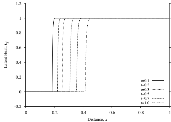
Figure 8: Model Problem 1: Evolution of latent heat (smooth interface), C^{11}(\bar{Q}_{st}^e) , p = 7 , \Delta t = 0.01
