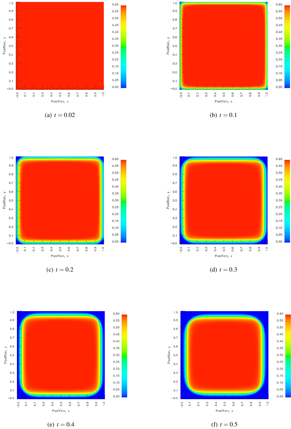
Figure 27: Model Problem 4: Evolution of latent heat for liquid-solid phase change in \mathbb{R}^2 , C^{00}(\bar{\Omega}_{\mathbf{x}}^e) , p = 3 , \Delta t = 0.0025 for 0 \leq t \leq 0.02 and \Delta t = 0.01 for t \geq 0.02
