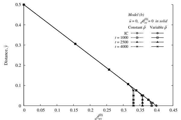
Figure 36: Model Problem 6: Evolution of d \bar{\tau}_{xy}^{(0)} versus \bar{y} using model (b), C^{11}(\bar{\Omega}_{\Delta t}^e) , p = 9, \Delta t = 50
