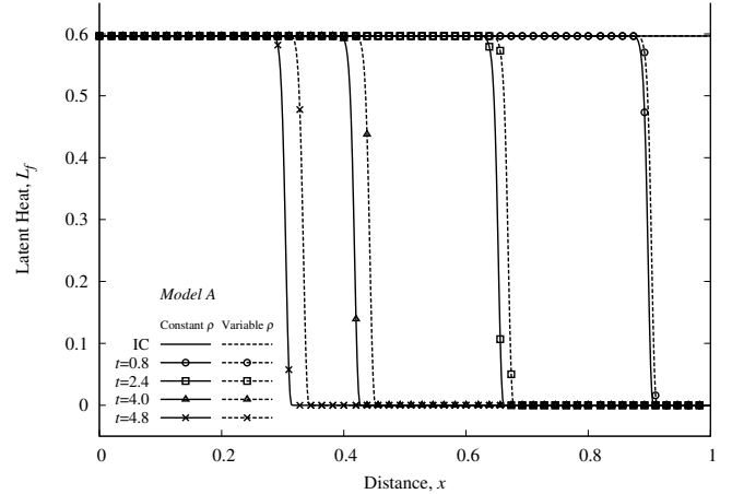
(b) Evolution of latent heat, 0.0 \leq t \leq 4.8
