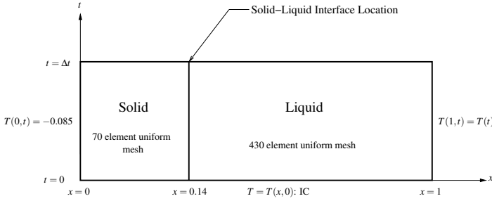
Figure 5: Schematic of first space-time strip, BCs, IC, and spatial discretization
