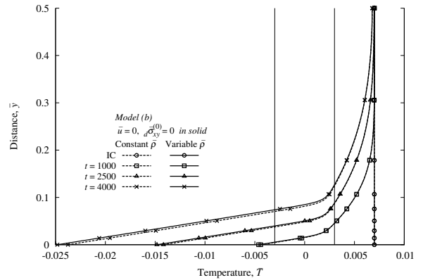
Figure 35: Model Problem 6: Evolution of temperature \bar{T} versus \bar{y} using model (b), C^{11}(\bar{\Omega}_{\Delta t}^e) , p = 9, \Delta t = 50
