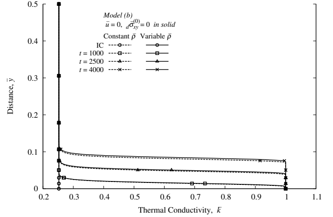
Figure 40: Model Problem 6: Evolution of thermal conductivity \bar{k} versus \bar{y} using model (b), C^{11}(\bar{\Omega}_{xt}^e) , p = 9, \Delta t = 50
