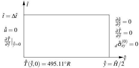
(a) Schematic of model problem 6
