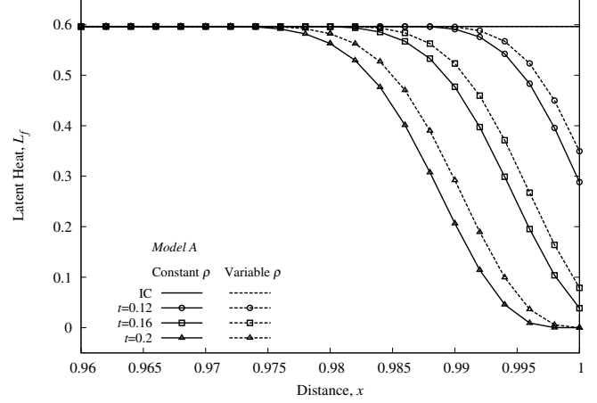
(a) Evolution of latent heat, 0.0 \leq t \leq 0.2
