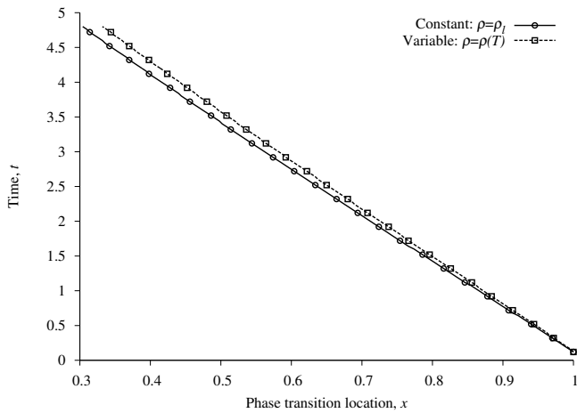
Figure 16: Model Problem 2: Interface location as a function of time, C^{11}(\bar{\Omega}_M^e) , p = 9, \Delta t = 0.04
