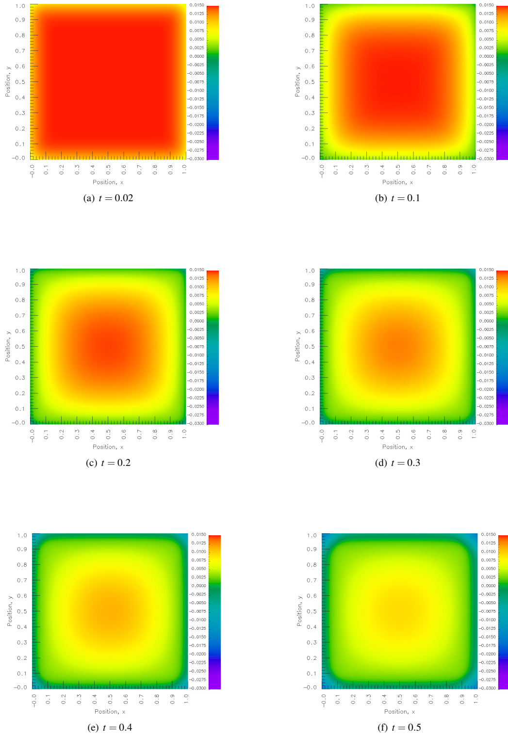
Figure 26: Model Problem 4: Evolution of temperature for liquid-solid phase change in \mathbb{R}^2 , C^{00}(\bar{\Omega}_{\mathbf{x}}^e) , p = 3 , \Delta t = 0.0025 for 0 \leq t \leq 0.02 and \Delta t = 0.01 for t \geq 0.02
