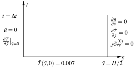
(b) Space-time strip
