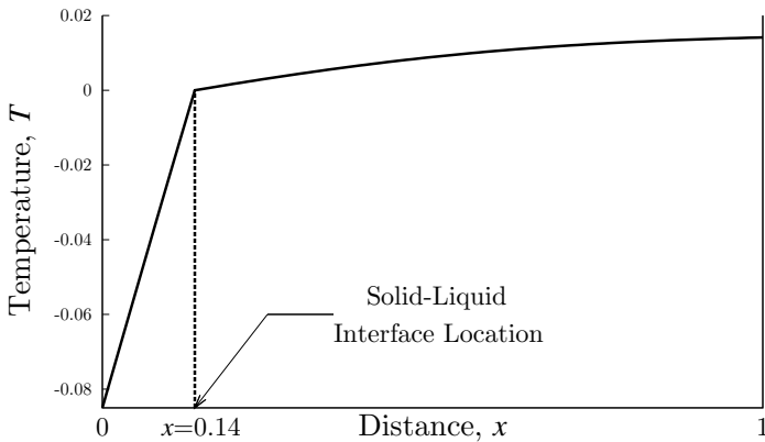
Figure 6: Initial condition \Theta(x) at t = 0 , temperature distribution from the theoretical solution of the sharp-interface model
