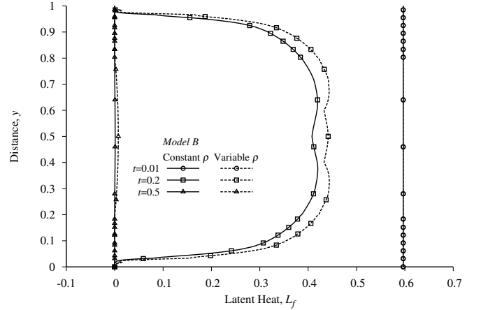
(b) Evolution of latent heat at the boundary
