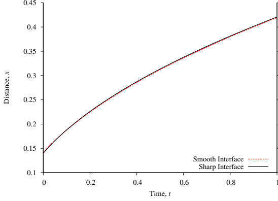
Figure 9: Model Problem 1: Interface location as a function of time, C^{11}(\bar{\Omega}_{\Delta t}^e), p = 7, \Delta t = 0.01
