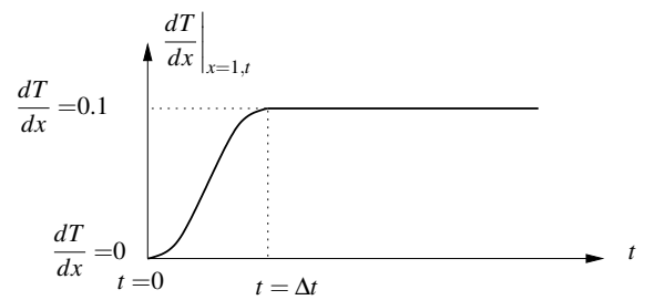
(c) Boundary condition \frac{dT}{dx} at x = 1
