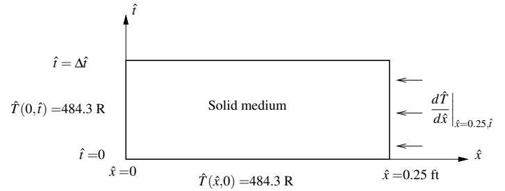
(a) Space-time strip
