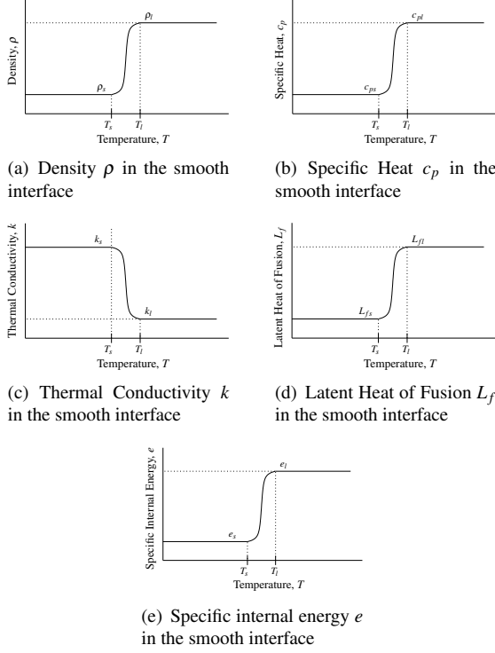
Figure 4: \rho , c_p , k , L_f and e in the smooth interface transition region between the solid and liquid phases as functions of Temperature T
