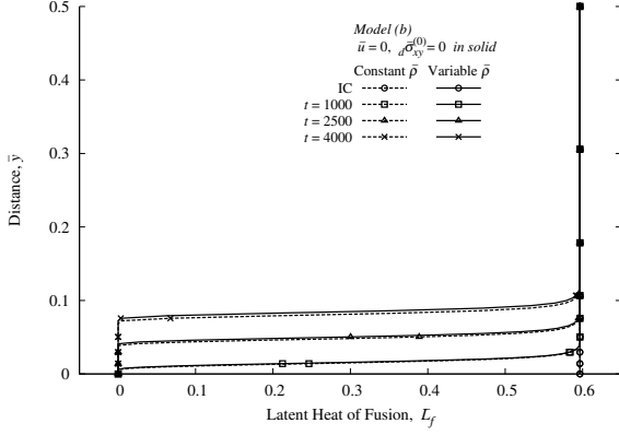
Figure 37: Model Problem 6: Evolution of latent heat \bar{L}_f versus \bar{y} using model (b), C^{11}(\bar{\Omega}_{xt}^e) , p = 9, \Delta t = 50
