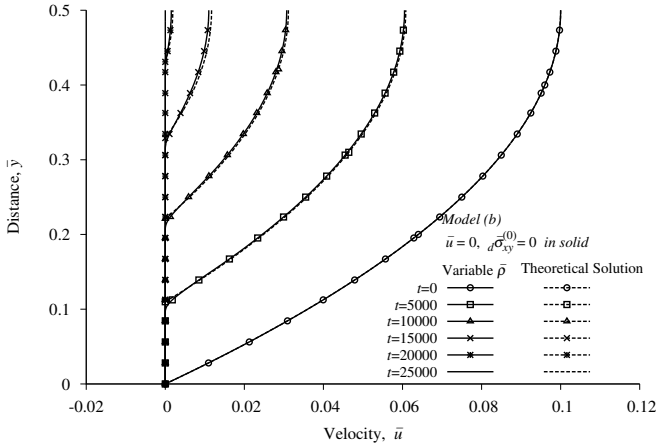
Figure 41: Model Problem 6: Evolution of velocity \bar{u} versus \bar{y} using model (b), C^{11}(\bar{\Omega}_{xt}^e) , p = 9, \Delta t = 50
