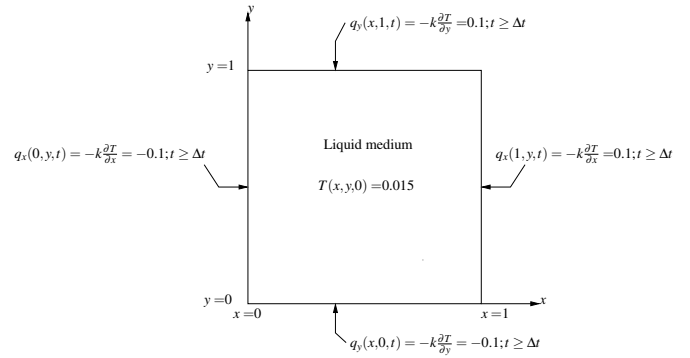
(b) Dimensionless space-time slab
