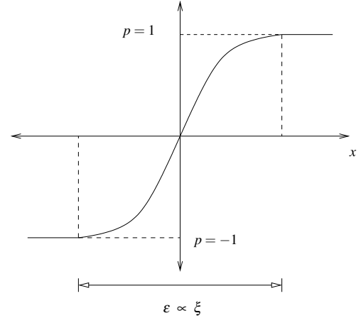
Figure 2: Expected spatial profile of phase field through a solid-liquid interface
