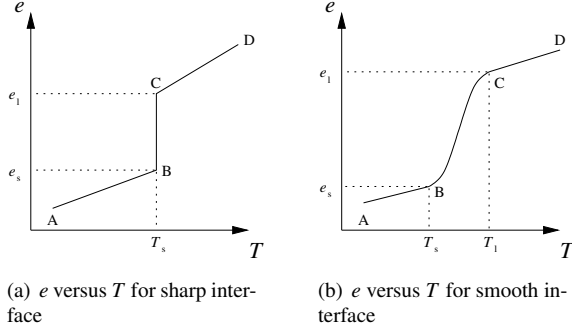
Figure 1: Sharp- and smooth-interface models for specific internal energy
