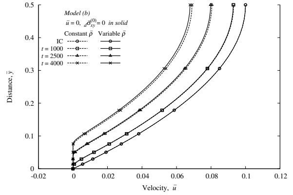
Figure 34: Model Problem 6: Evolution of velocity \bar{u} versus \bar{y} using model (b), C^{11}(\bar{\Omega}_{\Delta t}^e) , p = 9, \Delta t = 50
