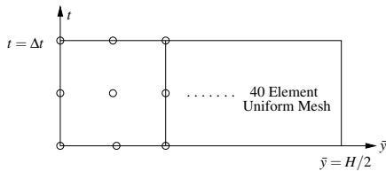
(e) Space-time discretization
