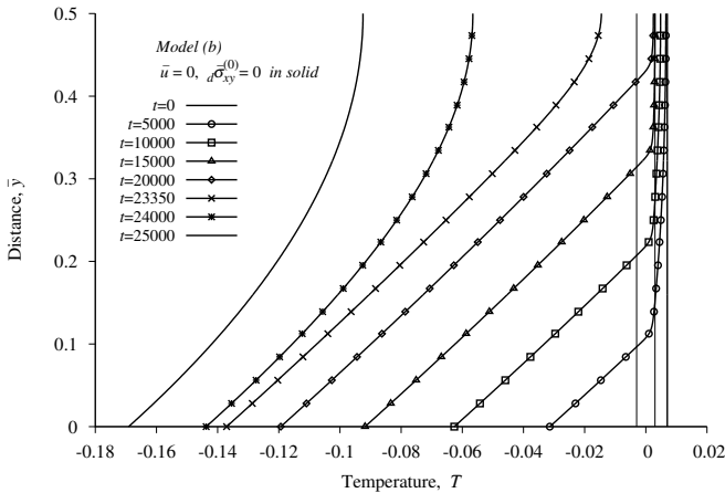
Figure 42: Model Problem 6: Evolution of temperature \bar{T} versus \bar{y} using model (b), C^{11}(\bar{\Omega}_{xt}^e) , p = 9, \Delta t = 50
