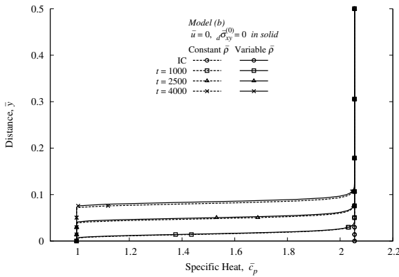
Figure 39: Model Problem 6: Evolution of specific heat \bar{c}_p versus \bar{y} using model (b), C^{11}(\bar{\Omega}_{xt}^e) , p = 9, \Delta t = 50
