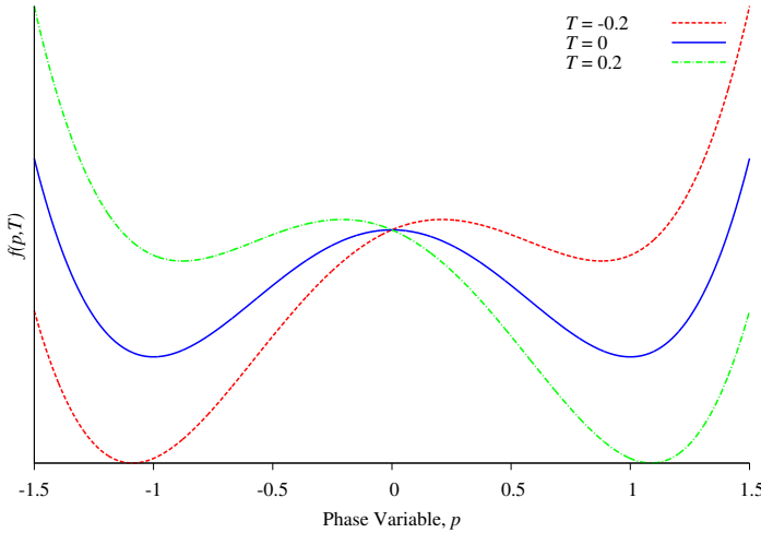
Figure 3: Double-well behavior of restoring potential for various values of temperature
