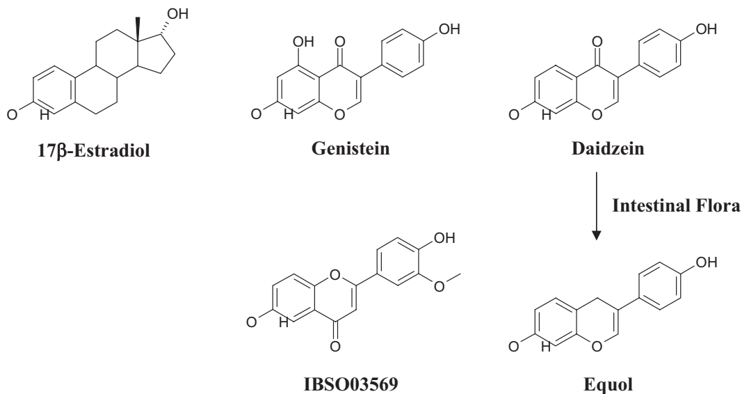
FIG. 1. Chemical structures of 17β-E2 and phytoestrogens tested in the present study. G and D are active aglycones of glucoside conjugates, genistein and daidzin, two main isoflavone constituents widely distributed in legumes such as soybeans. E is not of plant origin yet can be produced from D by enteric microfloral metabolism in a subset of human populations. I is a flavone derivative of D with an additional hydroxyl group attached to the 2-phenol ring.
