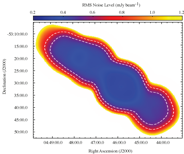
Figure 2. Noise map of the AzTEC/ASTE ADF-S. The outer and inner contours indicate the 30 and 50 per cent coverage regions, respectively.
