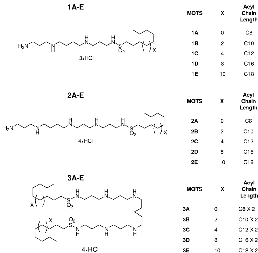
FIG. 2. Structures of the polyamine sulfonamides.
