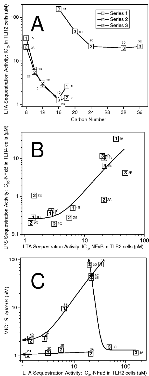
FIG. 4. (A) Correlation of carbon number of the acyl chain of the polyamine sulfonamides and their LTA-inhibitory activities, as assessed by the HEK-2-Blue NF- \kappa B reporter gene assay. (B) Correlation of inhibition of LTA- and LPS-induced NF- \kappa B translocation, as measured with HEK-2-Blue and HEK-4-Blue cells, respectively. Each dilution was tested in quadruplicate, and experiments were repeated three times; coefficients of variation were less than 7%, and for clarity, only the means are shown. (C) Correlation of LTA-inhibitory activity and activity against S. aureus strain ATCC 13709.
