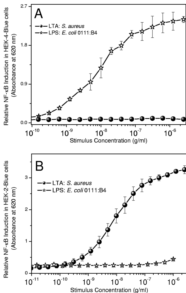
FIG. 3. (A) NF- \kappa B induction activity of LPS and LTA in TLR4-expressing HEK-4-Blue cells treated overnight. sAP was measured colorimetrically. (B) NF- \kappa B induction in TLR2-expressing HEK-2-Blue cells treated overnight with 1:2 serially diluted concentrations of LPS and LTA ascertained as described for panel A. Each dilution was tested in quadruplicate; coefficients of variation were less than 3%, and for clarity, only the means are shown.
