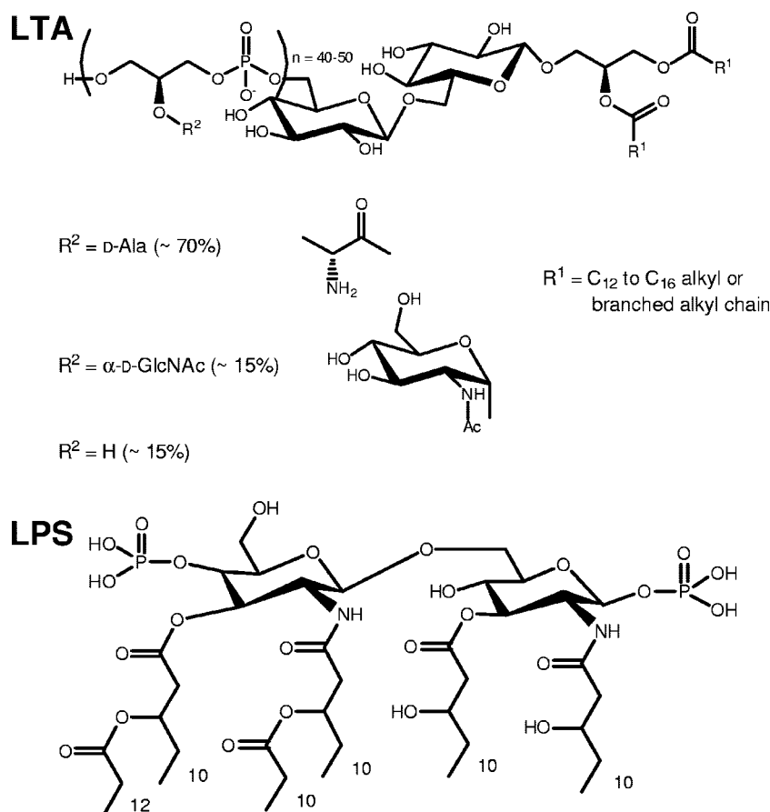
FIG. 1. Structures of LTA and LPS showing physicochemical similarities (anionic amphipathic molecules).
