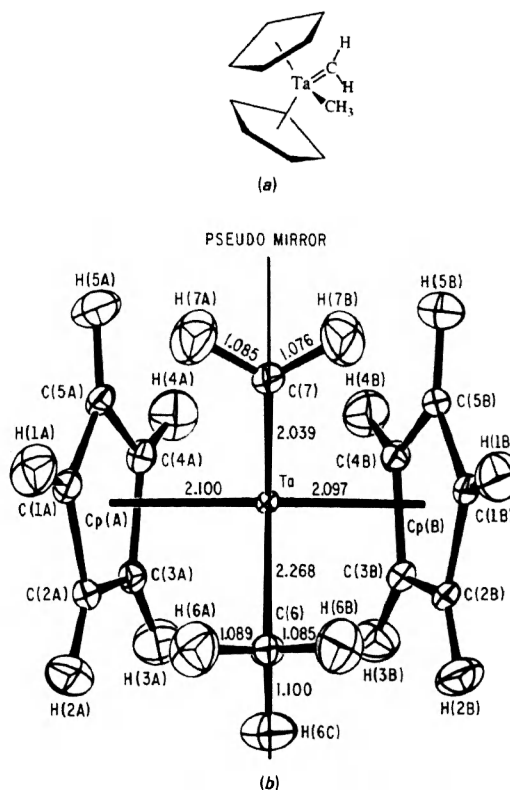
Fig. 1. (a) Schematic drawing of [\text{Ta}(\eta^5\text{-C}_5\text{H}_5)_2(\text{CH}_2)(\text{CH}_3)] . (b) View showing the atom numbering and essential bond distances. Thermal ellipsoids are drawn at the 50% probability level (Johnson, 1976).
