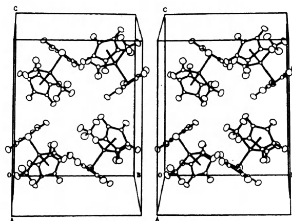
Fig. 2. Stereoview of [\text{Ta}(\eta^5\text{-C}_5\text{H}_5)_2(\text{CH}_2)(\text{CH}_3)] , viewed down c , with ellipsoids as in Fig. 1(b).
